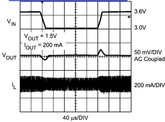
Line Transient Response 查询"LM3280"供应商
