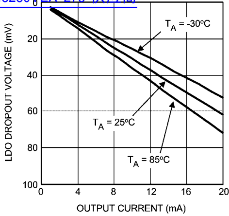
LDO Dropout Voltage vs Output Current 查询"LM3280TLX-275"供应商
