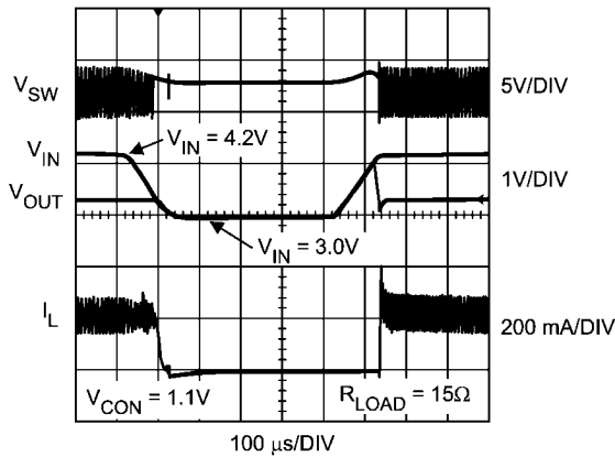
Automatic Bypass Operation (V_{IN} = 4.2V \text{ to } 3.0V)
