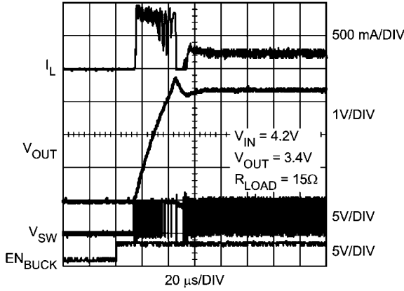
PWM Startup (V_{CON} = 1.13V)
