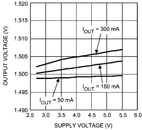
PWM Output Voltage vs Supply Voltage 查询"LM3280(V_X-275V)供应商
