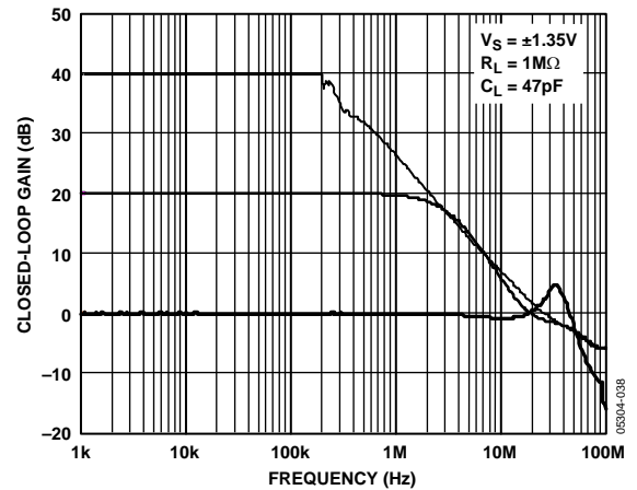
Figure 52. Closed-Loop Gain vs. Frequency
