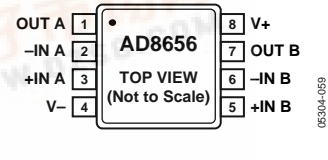
Figure 2. AD8656 8-Lead MSOP (RM-8)
