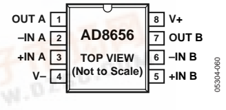
Figure 4. AD8656 8-Lead SOIC (R-8)
