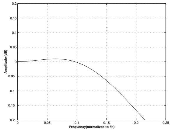
Figure 38. Quad-Speed (fast) Passband Ripple
