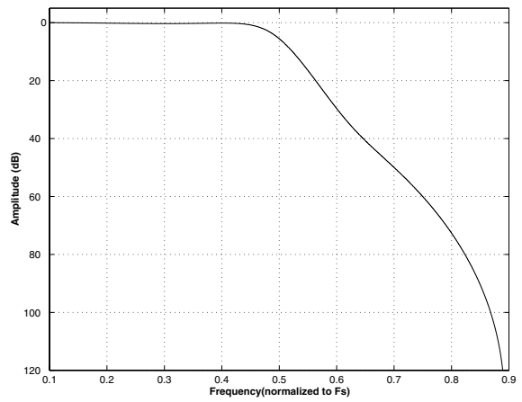
Figure 40. Quad-Speed (slow) Transition Band
