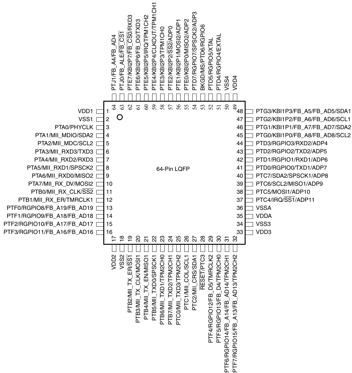
Figure 3. Pin Assignments in 64-Pin LQFP Package
