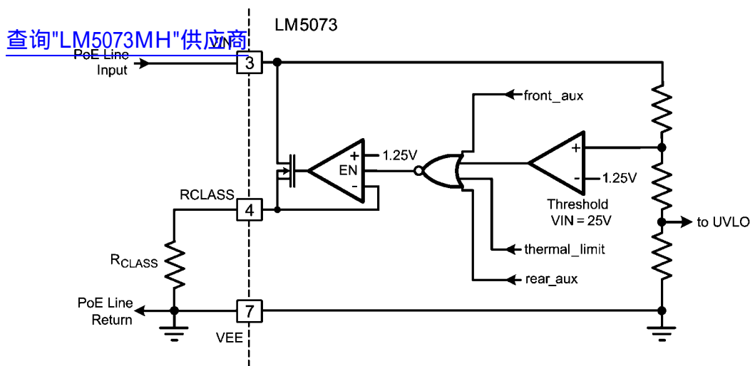
FIGURE 4. PD Classification – Fulfilled With a Single External Resistor
