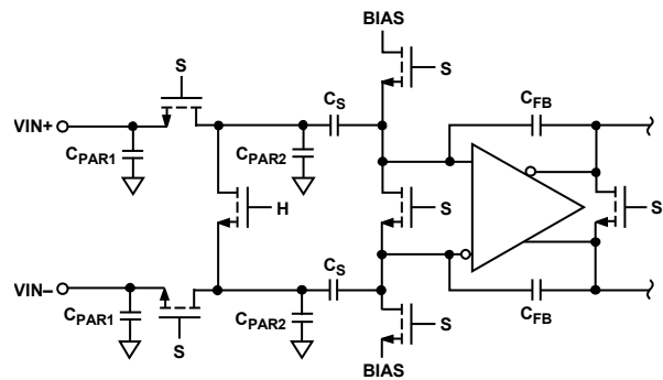
Figure 29. Switched-Capacitor Input
