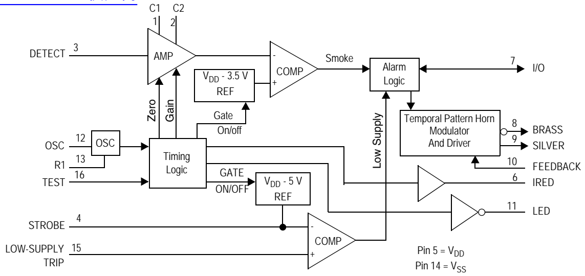
Figure 2. Block Diagram
