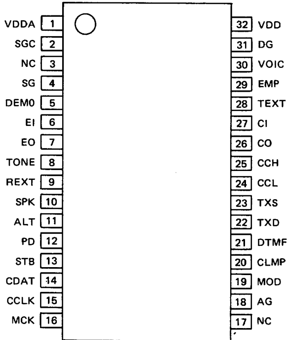
32 PIN Plastic Flat PKG
