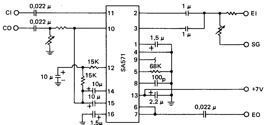
Figure 6 Comparator.
