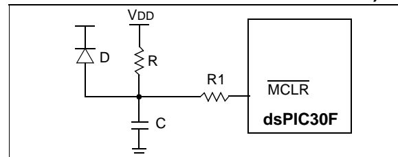
FIGURE 18-10: EXTERNAL POWER-ON RESET CIRCUIT (FOR SLOW VDD POWER-UP)
