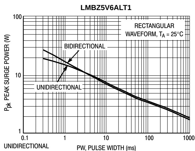
Figure 8. Maximum Non-repetitive Surge Power, P_{pk(NOM)} versus PW
