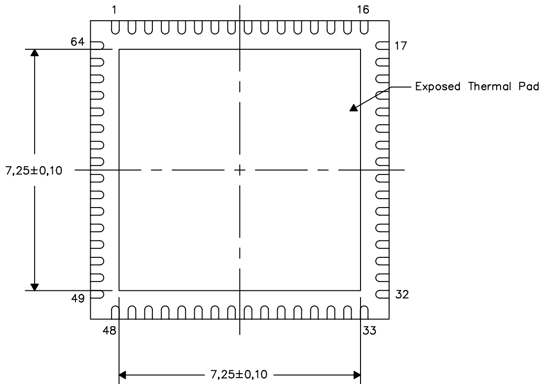
Bottom View
