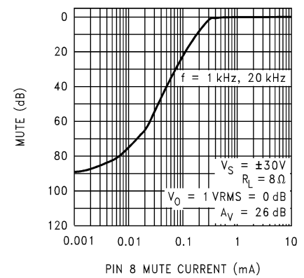
Mute Attenuation vs Mute Current
