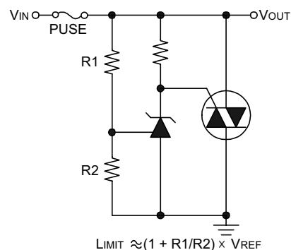
Fig.6 Crow Bar
