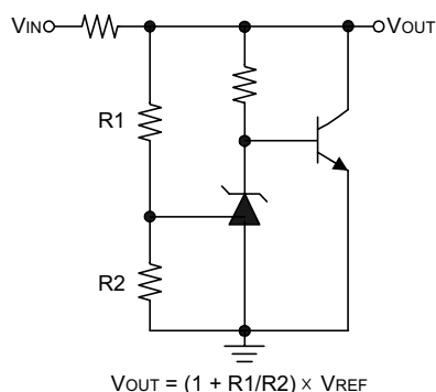
Fig.5 Higher-Current Shunt Regulator
