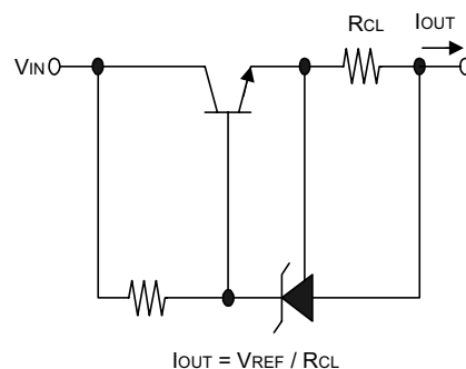
Fig.3 Current Limiter or Current Source
