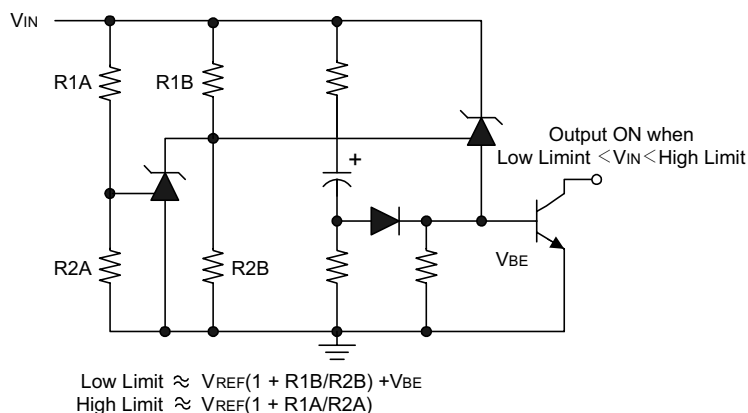
Fig.7 Over-Voltage / Under-Voltage Protection Circuit
