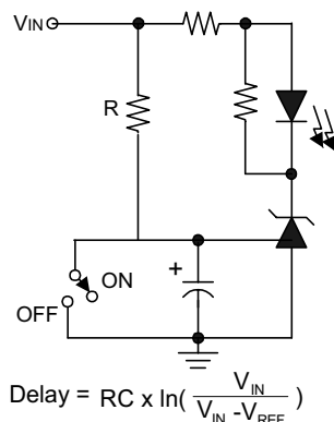
Fig.2 Delay Timer
