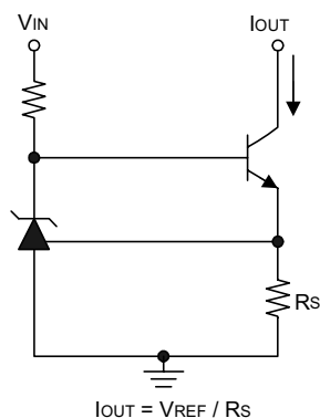
Fig.4 Constant-Current Sink
