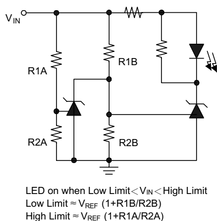
Fig.1 Voltage Monitor
