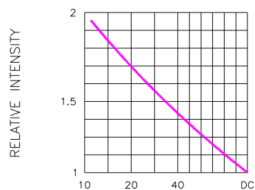
Fig.5 LUMINOUS INTENSITY VS. DUTY CYCLE (AVERAGE If=10mA)
