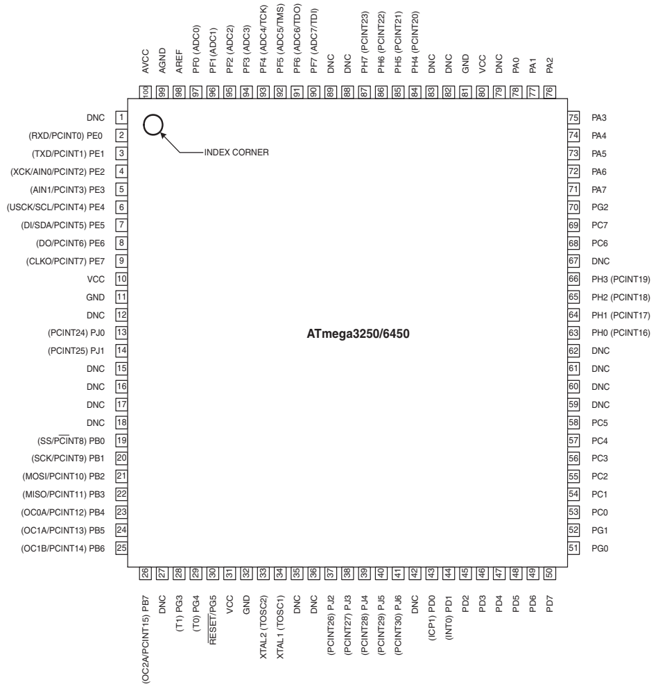
Figure 1. Pinout ATmega3250/6450
