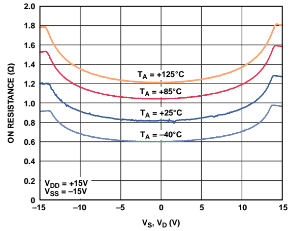
Figure 7. On Resistance as a Function of V_D ( V_S ) for Different Temperatures, \pm 15 V Dual Supply
