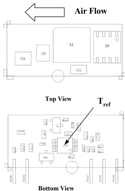
Figure 32. T_{ref} Temperature measurement location.
