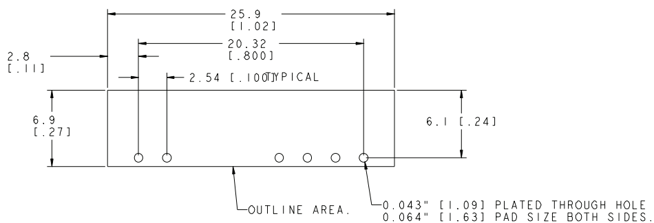
Through-Hole Pad Layout – Back view
