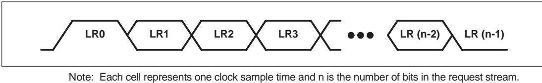
Figure 13. LREQ Request Stream
