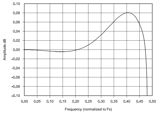
Figure 27. Passband Ripple
