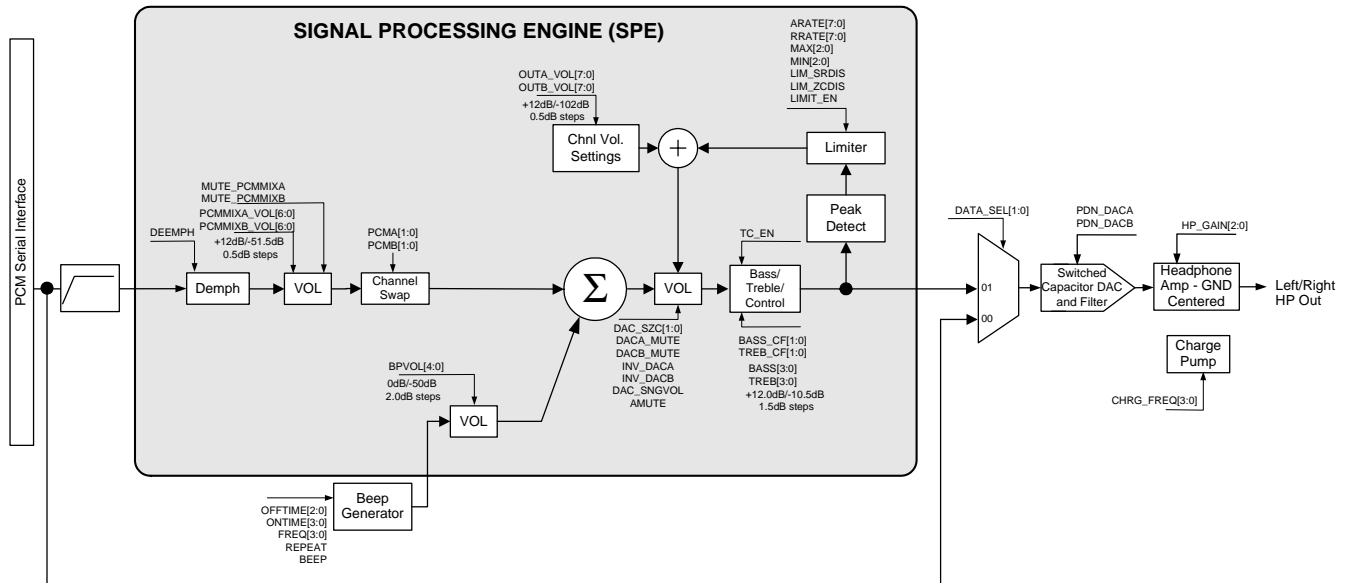
Figure 8. Output Architecture
