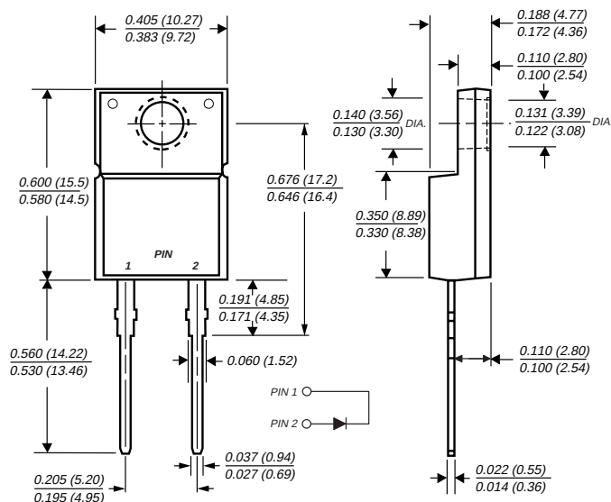
ITO-220AC (MBRF7Hxx)
