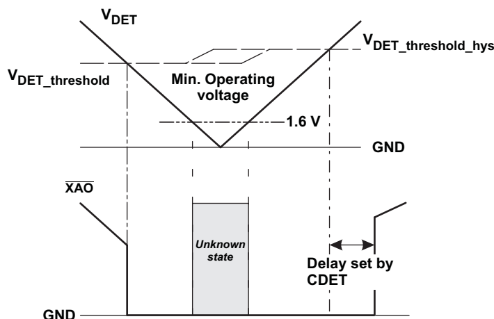
Figure 25. Voltage Detection and XAO Pin
