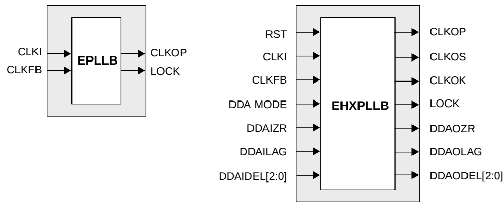
Figure 2-12. PLL Primitive
