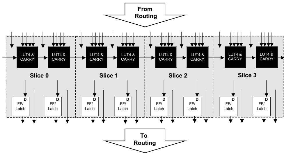
Figure 2-3. PFU Diagram
