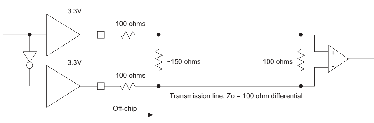
Figure 3-2. Differential LVPECL
