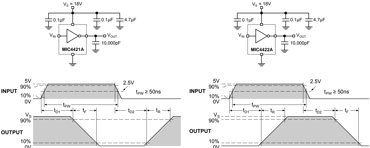
Figure 1. Inverting Driver Switching Time
