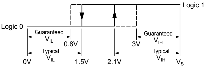
Figure 3. Input Hysteresis
