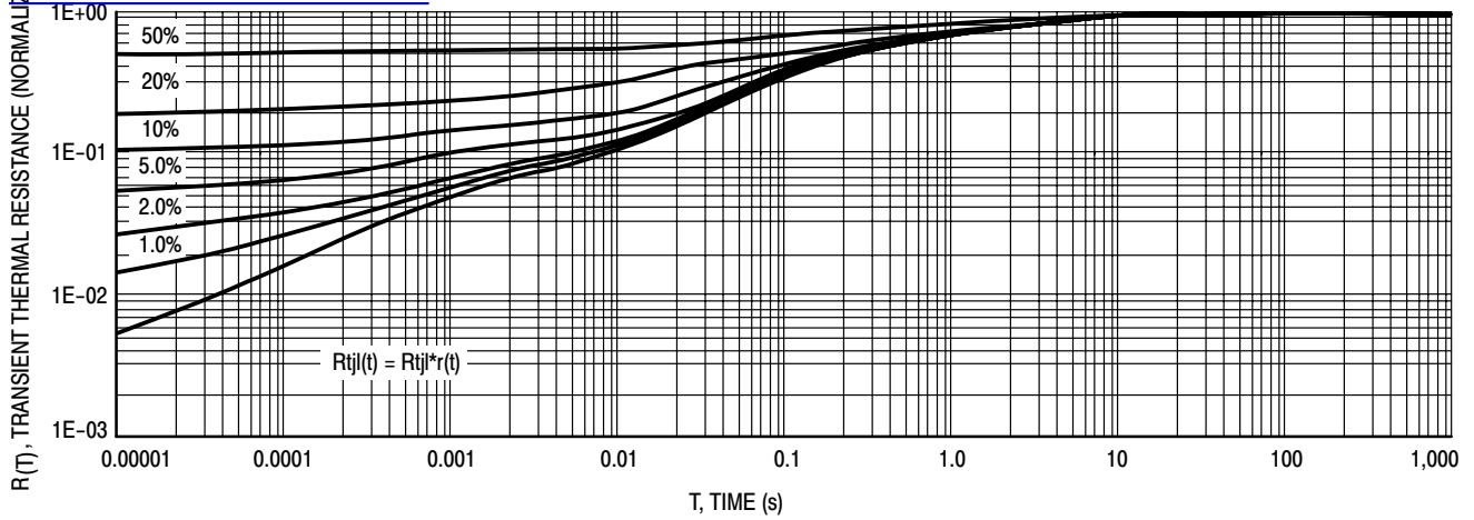
Figure 9. Thermal Response Junction to Lead
