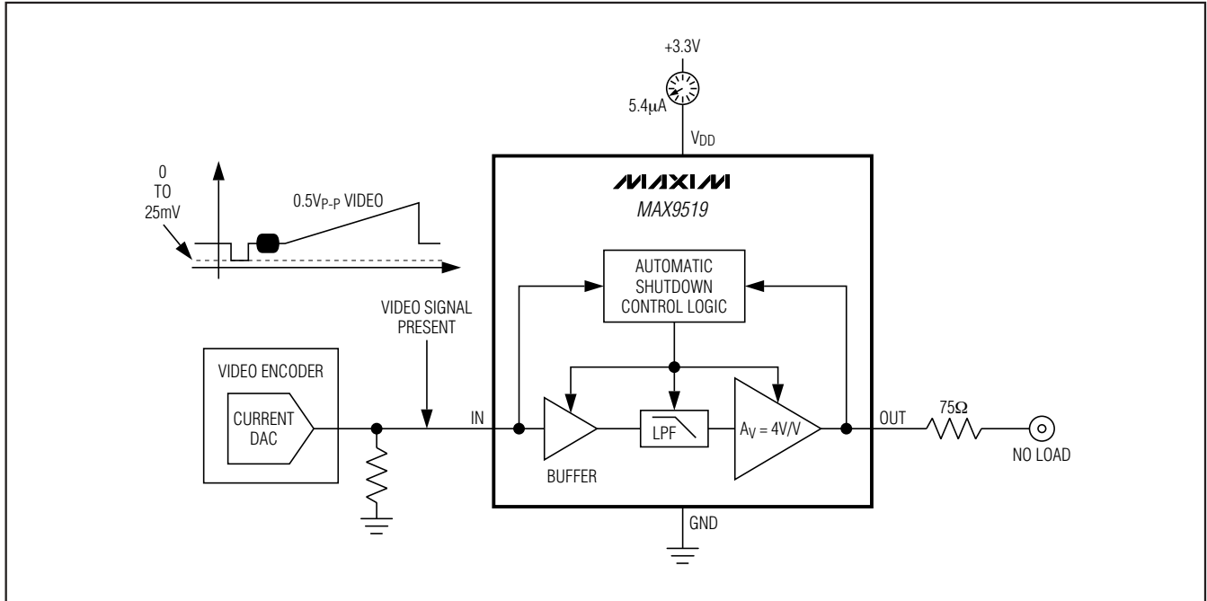
Figure 2. Active-Detect Mode
