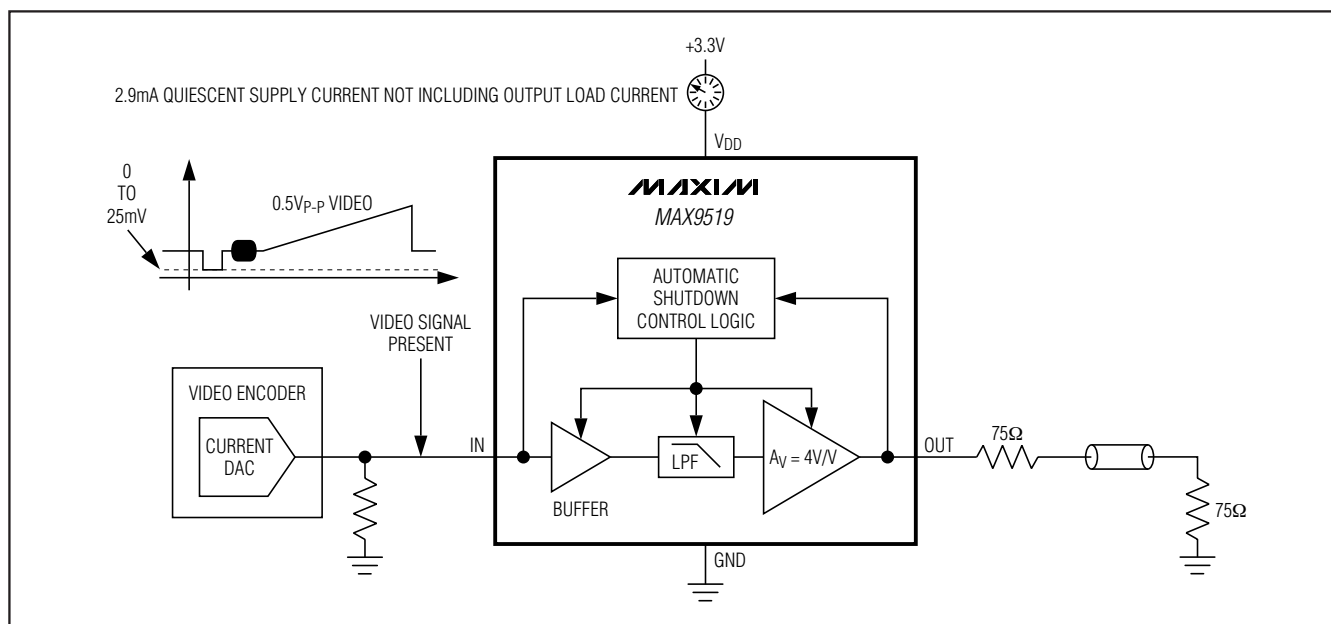
Figure 3. Full-Operation Mode
