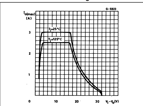
Figure 9. Peak output current vs input/output differential voltage
