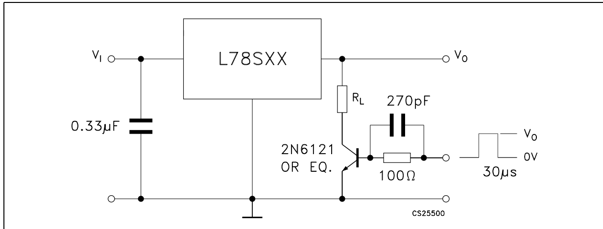
Figure 6. Load regulation
