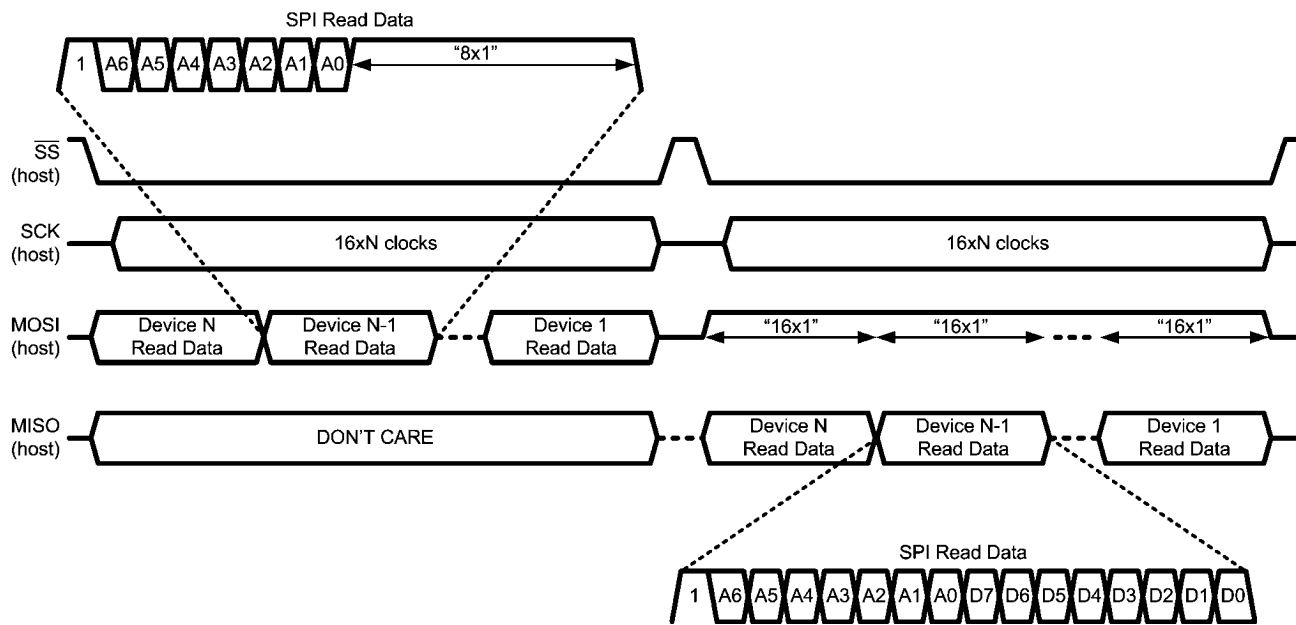
FIGURE 9. SPI Daisy-Chain Read
