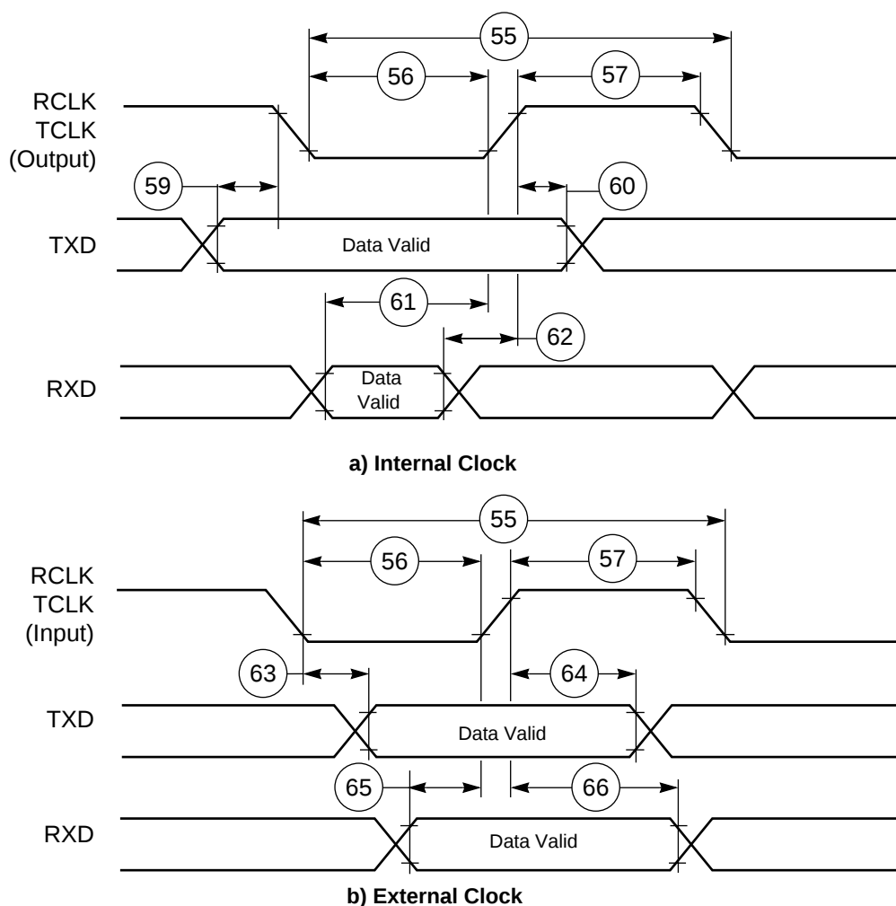
Figure 2-17 SCI Synchronous Mode Timing
