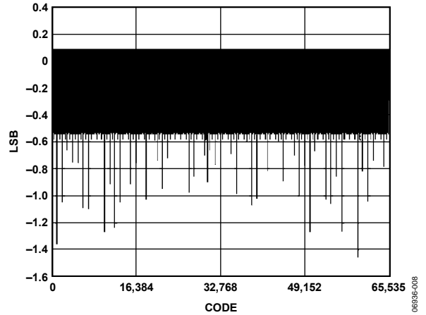
Figure 8. AD9783 DNL, T_A = 85^\circ\text{C} , FS = 20\text{ mA}
