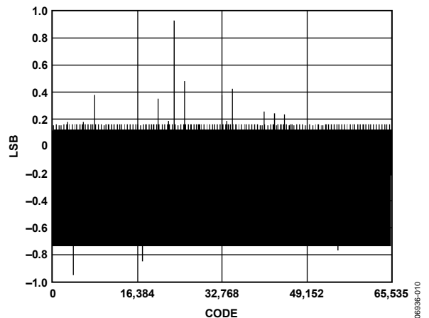
Figure 10. AD9783 DNL, T_A = -40^\circ\text{C} , FS = 20\text{ mA}
