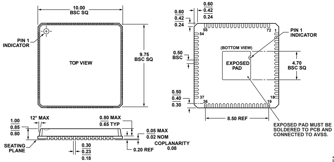
COMPLIANT TO JEDEC STANDARDS MO-220-VNND-4 Figure 79. 72-Lead Lead Frame Chip Scale Package [LFCSP_VQ] 10 mm × 10 mm, Very Thin Quad (CP-72-1) Dimensions shown in millimeters
