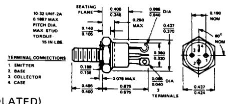
TO-111 (ISOLATED)
