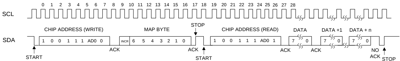
Figure 22. Control Port Timing, I²C Aborted Write + Read
