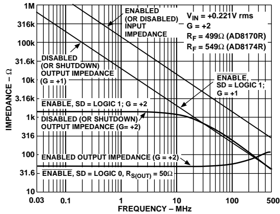
Figure 17. Input &amp; Output Impedance vs. Frequency
