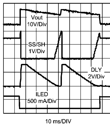
FIGURE 12. OVP and Auto-Restart
