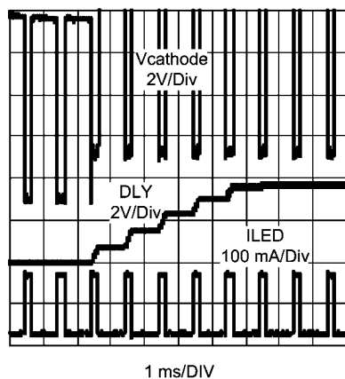
FIGURE 11. DLY Charging, 1 LED Open Fault
