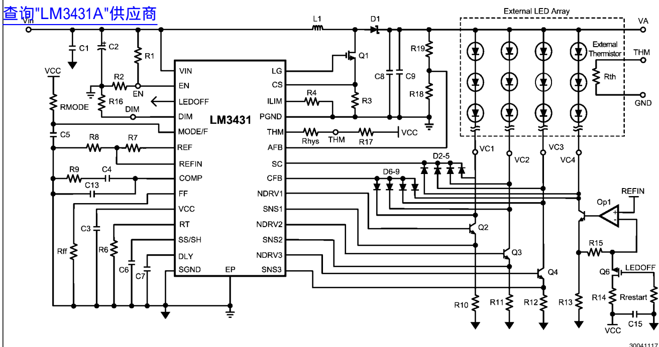
FIGURE 1. Typical Application Schematic
