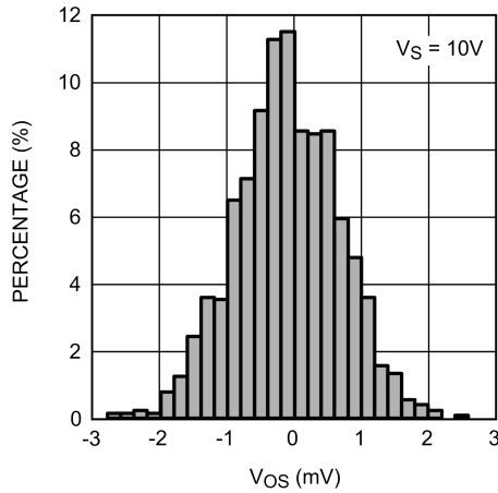
V_{OS} Distribution
