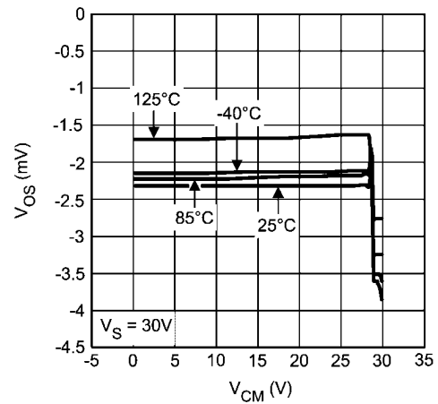
V_{OS} vs. V_{CM} (Unit 2)
