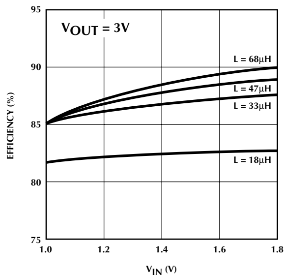
Figure 5. Typical Efficiency as a Function of V_{IN}
