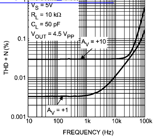
THD+N vs. Frequency 查询"LMV841 0710"供应商
