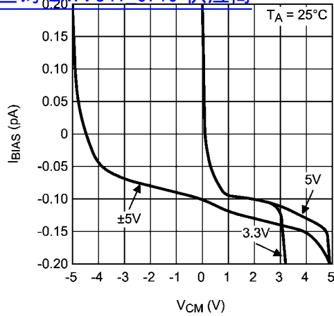
Input Bias Current vs. V_{CM} 查询"LMV841 0710"供应商
