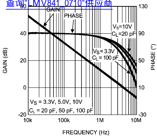
Open Loop Frequency Response Over Load Conditions
