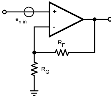
FIGURE 3. Noise Circuit
