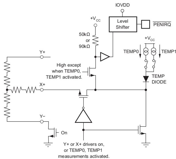
Figure 10. PENIRQ Functional Block Diagram
