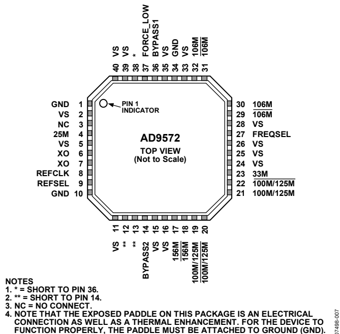
Figure 6. Pin Configuration
