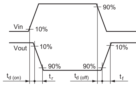
Waveforms
