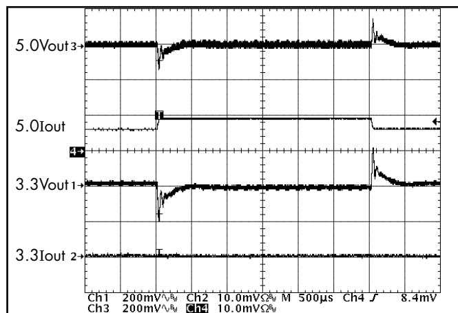
Figure 22: Output voltage response to step-change in Iout2 (50%-75%-50% of Imax; dI/dt = 0.1A/μs). Load cap: 15μF, 300 mΩ ESR tantalum cap & 1μF ceramic cap.. Vout (200mV/div), Iout (10A/div). Ch1:Vout1; Ch2:Iout1; Ch3:Vout2; Ch4:Iout2
