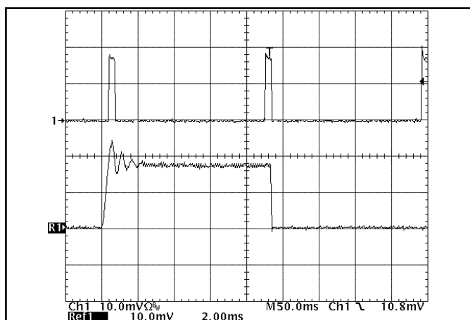
Figure 29: Load current for 3.3V output (10A/div) as a function of time when the converter attempts to turn on into a 10 m \Omega short circuit. Bottom trace is an expansion of the on-time portion of the top trace.
