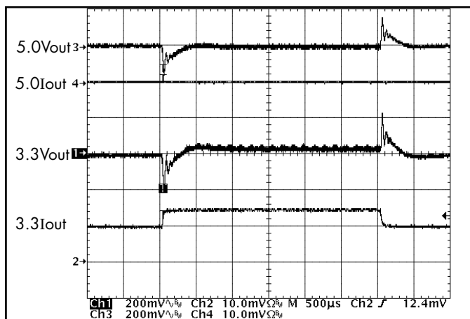
Figure 21: Output voltage response to step-change in Iout1 (50%-75%-50% of Imax; dI/dt = 0.1A/μs). Load cap: 15μF, 300 mΩ ESR tantalum cap & 1μF ceramic cap. Vout (200mV/div), Iout (10A/div). Ch1:Vout1; Ch2:Iout1; Ch3:Vout2; Ch4:Iout2
