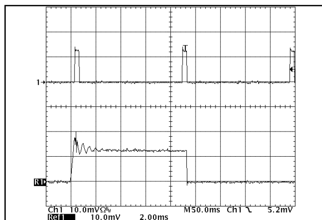
Figure 30: Load current for 5.0V output (10A/div) as a function of time when the converter attempts to turn on into a 10 m \Omega short circuit. Bottom trace is an expansion of the on-time portion of the top trace.
