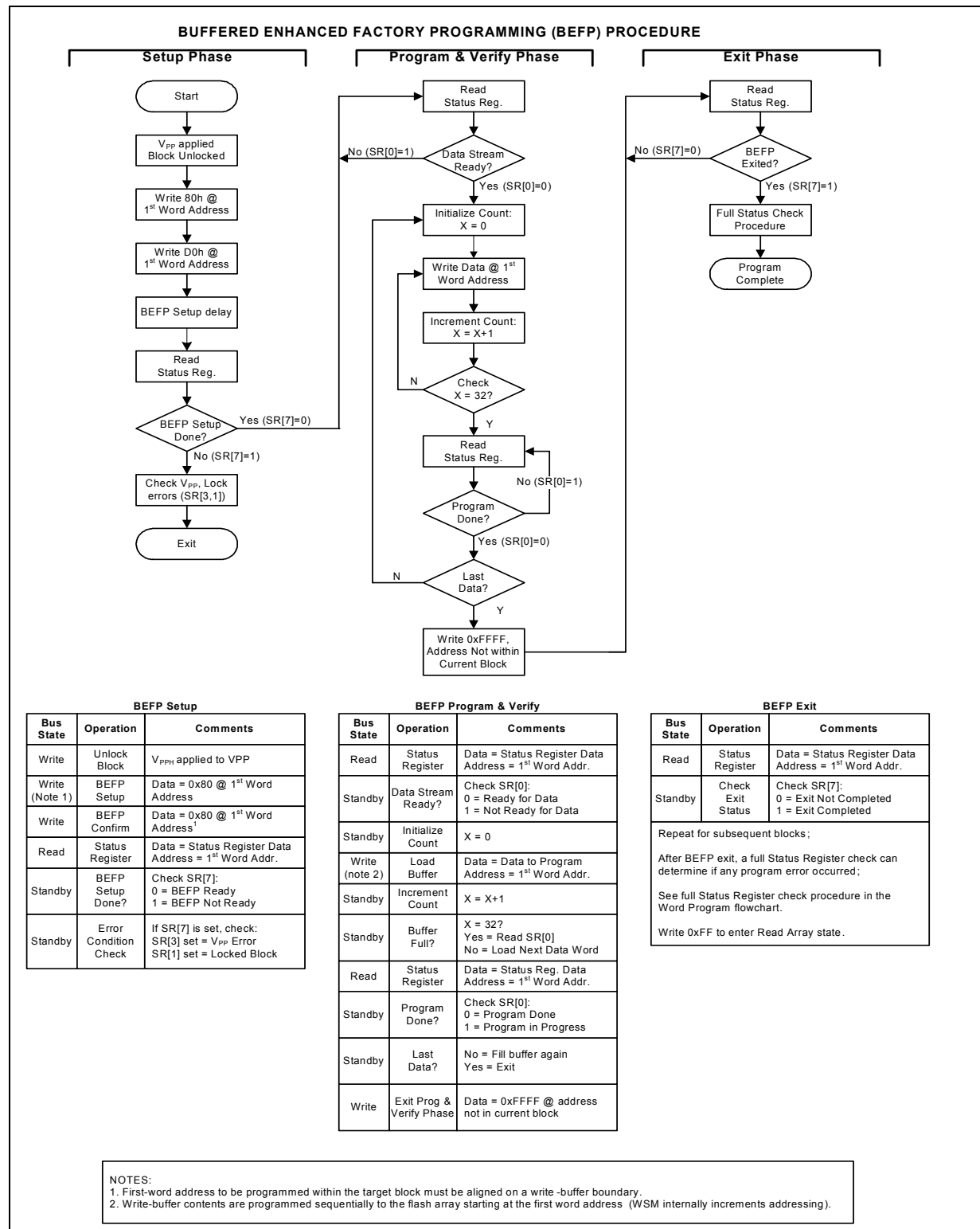
Figure 41: BEFP Flowchart
