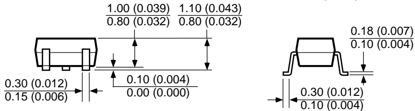
SC-70 (C5)
