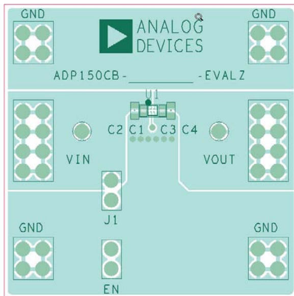
Figure 48. Example WLCSP PCB Layout
