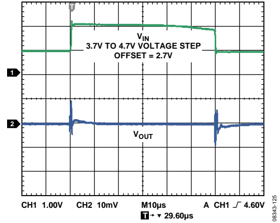
Figure 25. Line Transient Response, C_{IN}, C_{OUT} = 1 \mu F, I_{LOAD} = 150 \text{ mA}
