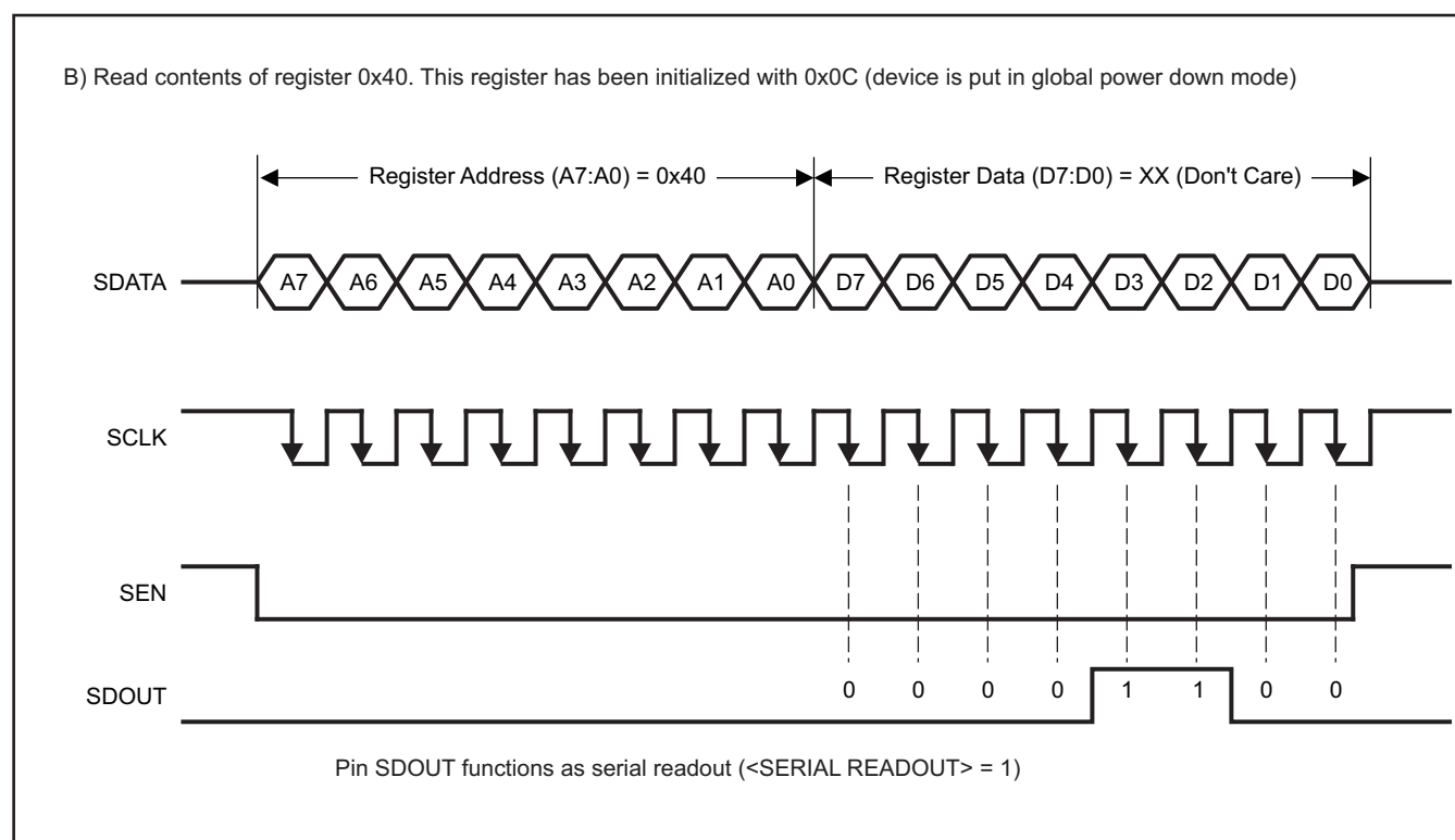
Figure 9. Serial Readout
