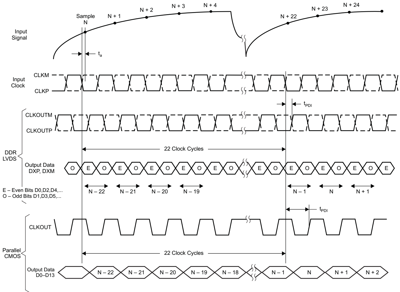
Figure 4. Latency Diagram
