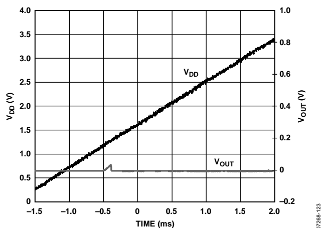
Figure 23. V DD and V OUT vs. Time on Power-Up
