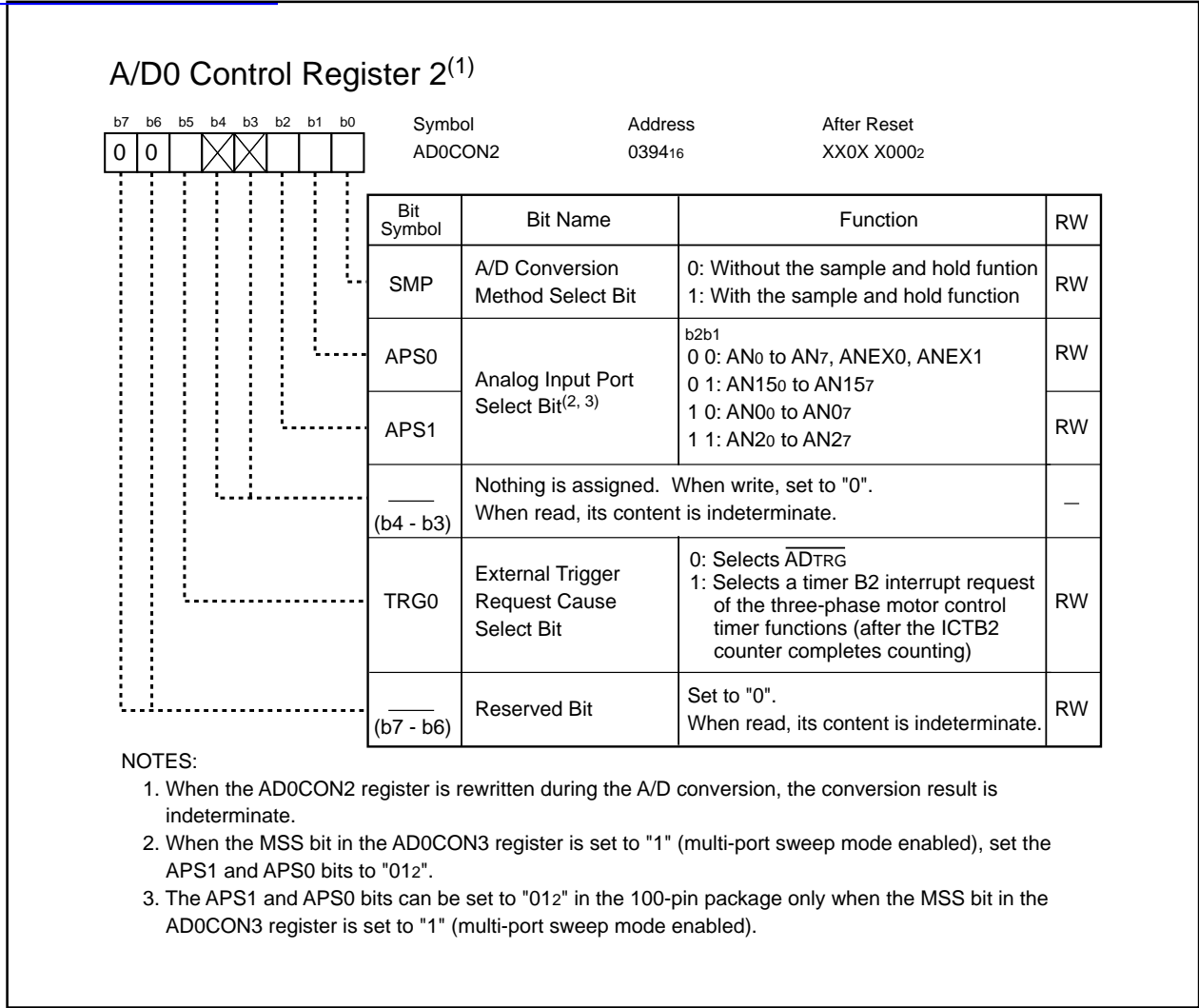
Figure 17.4 AD0CON2 Register
