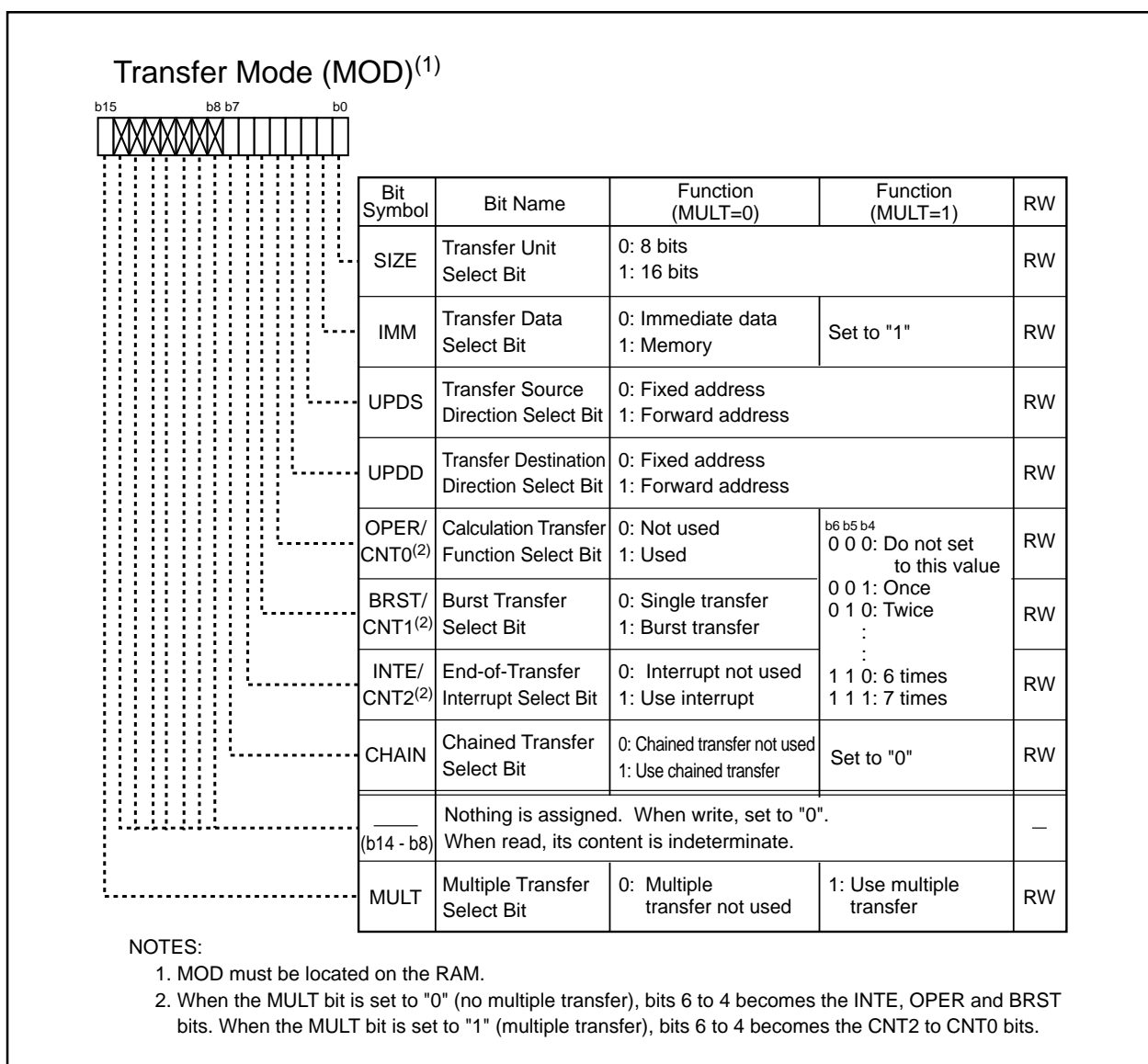
Figure 13.3 MOD
