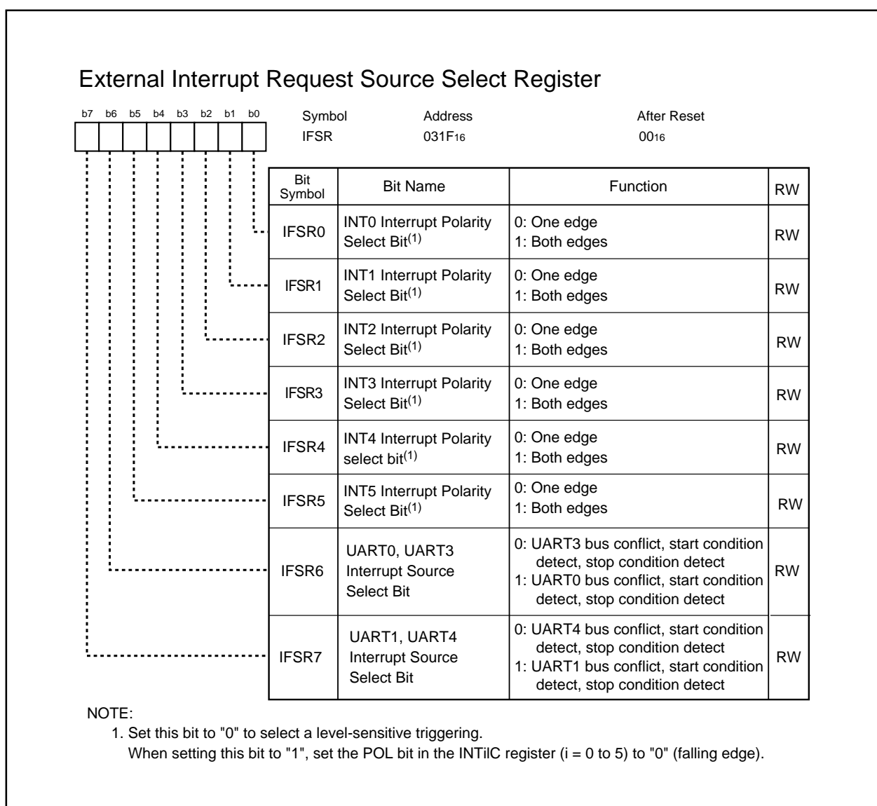
Figure 10.10 IFSR Register
