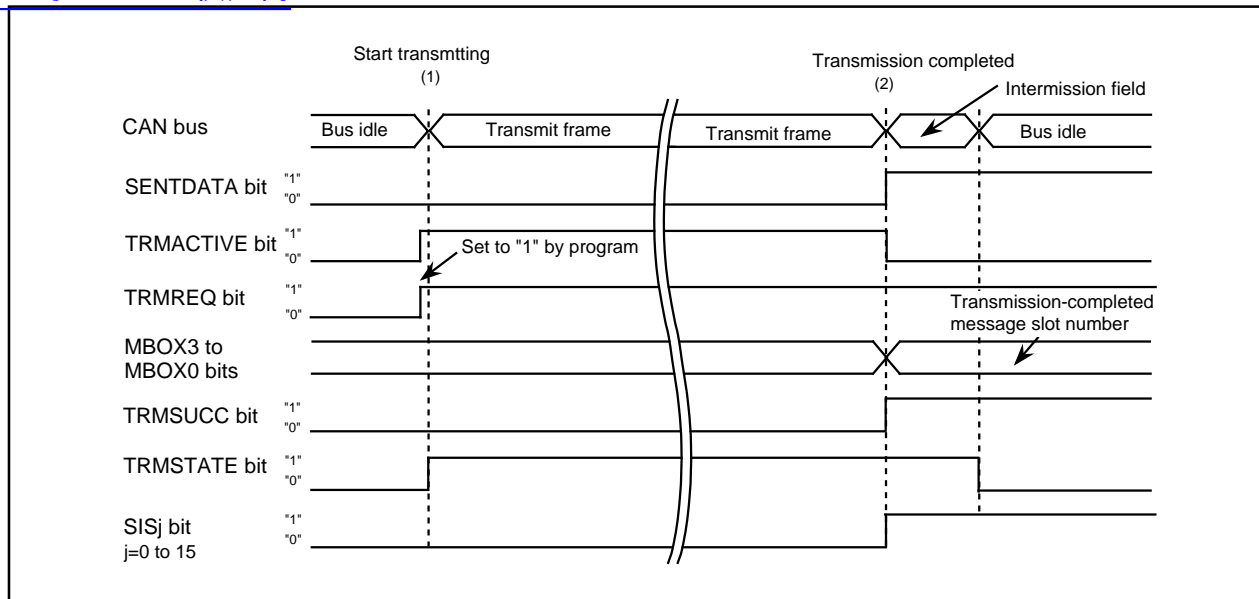
Figure 22.38 Example of CAN Data Frame Transmit Operation
