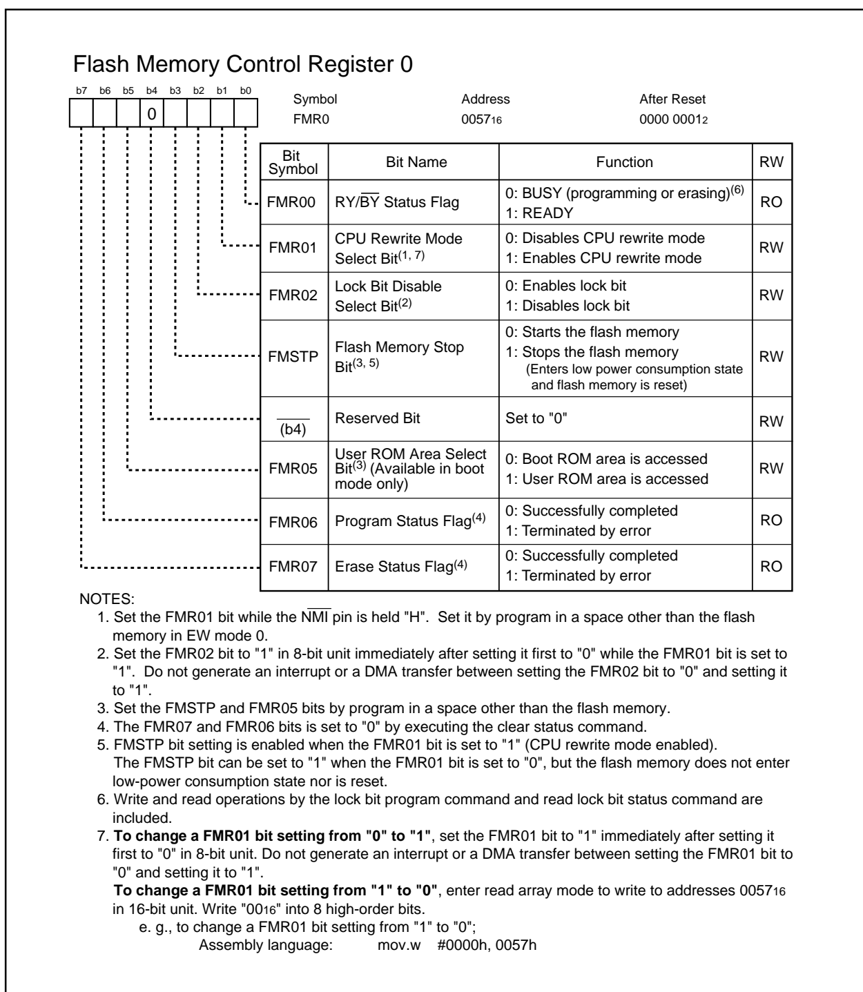
Figure 24.4 FMR0 Register
