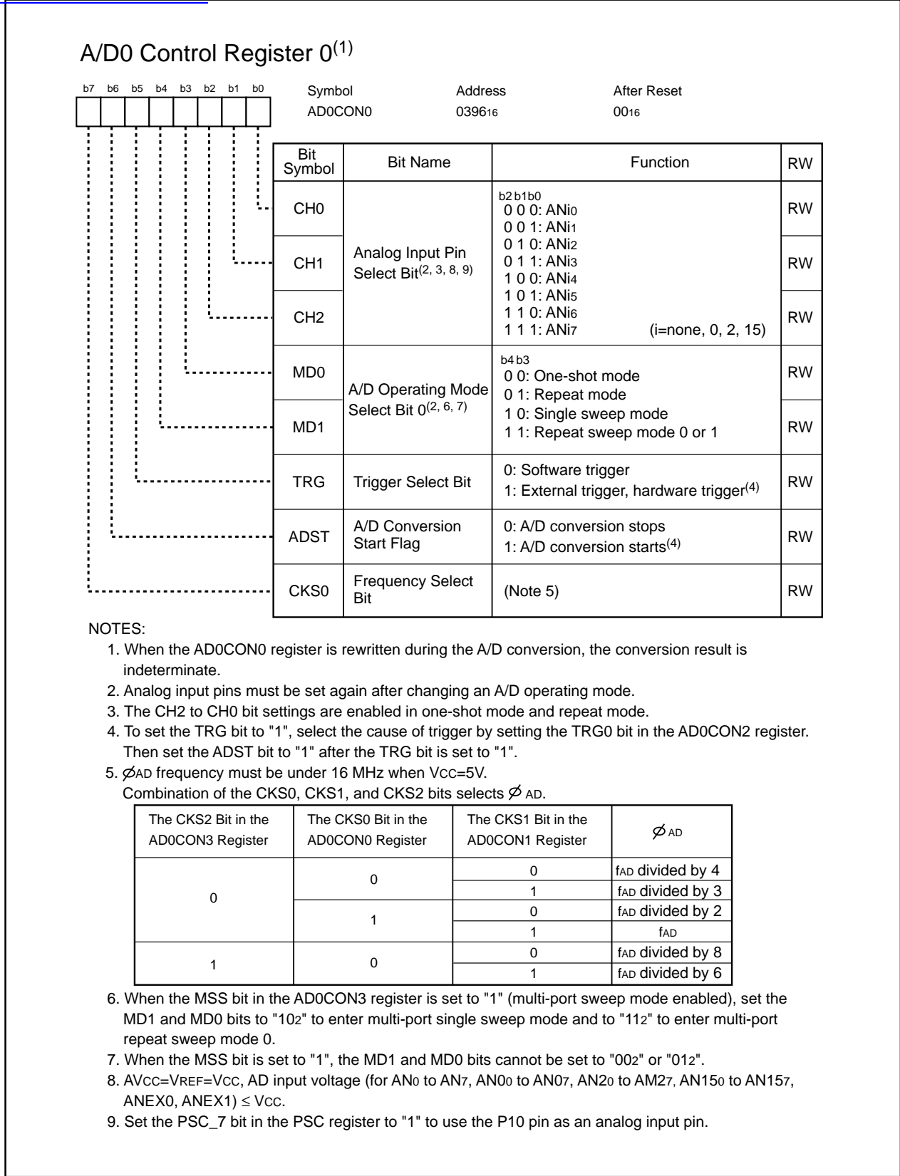
Figure 17.2 AD0CON0 Register
