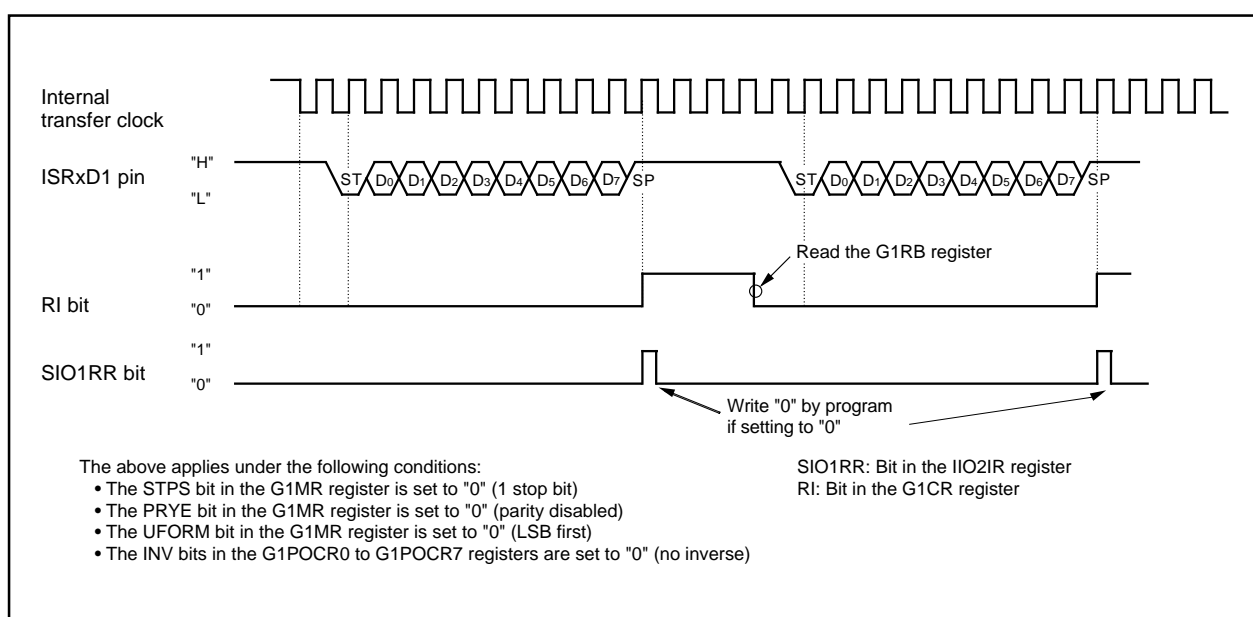
Figure 21.31 Receive Operation
