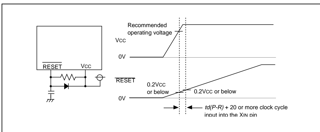
Figure 5.1 Reset Circuit
