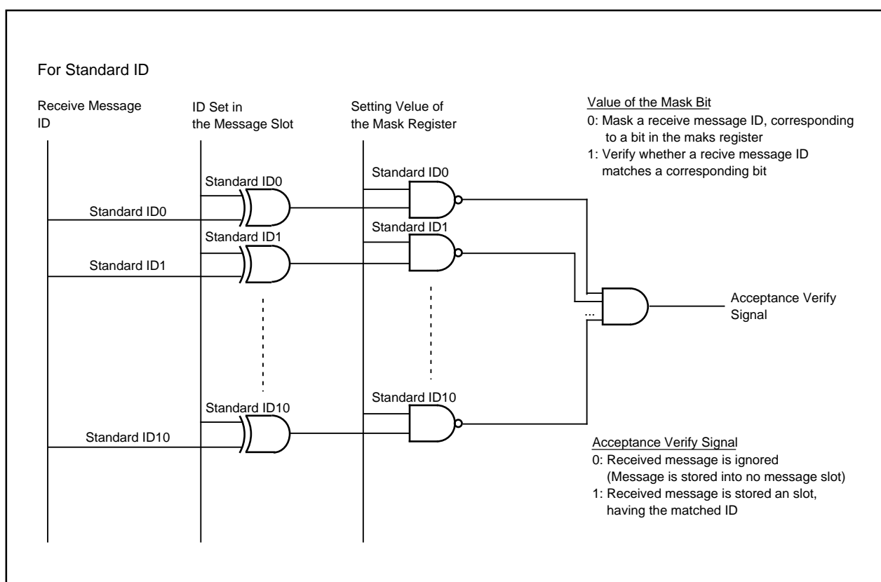
Figure 22.28 Acceptance Filtering
