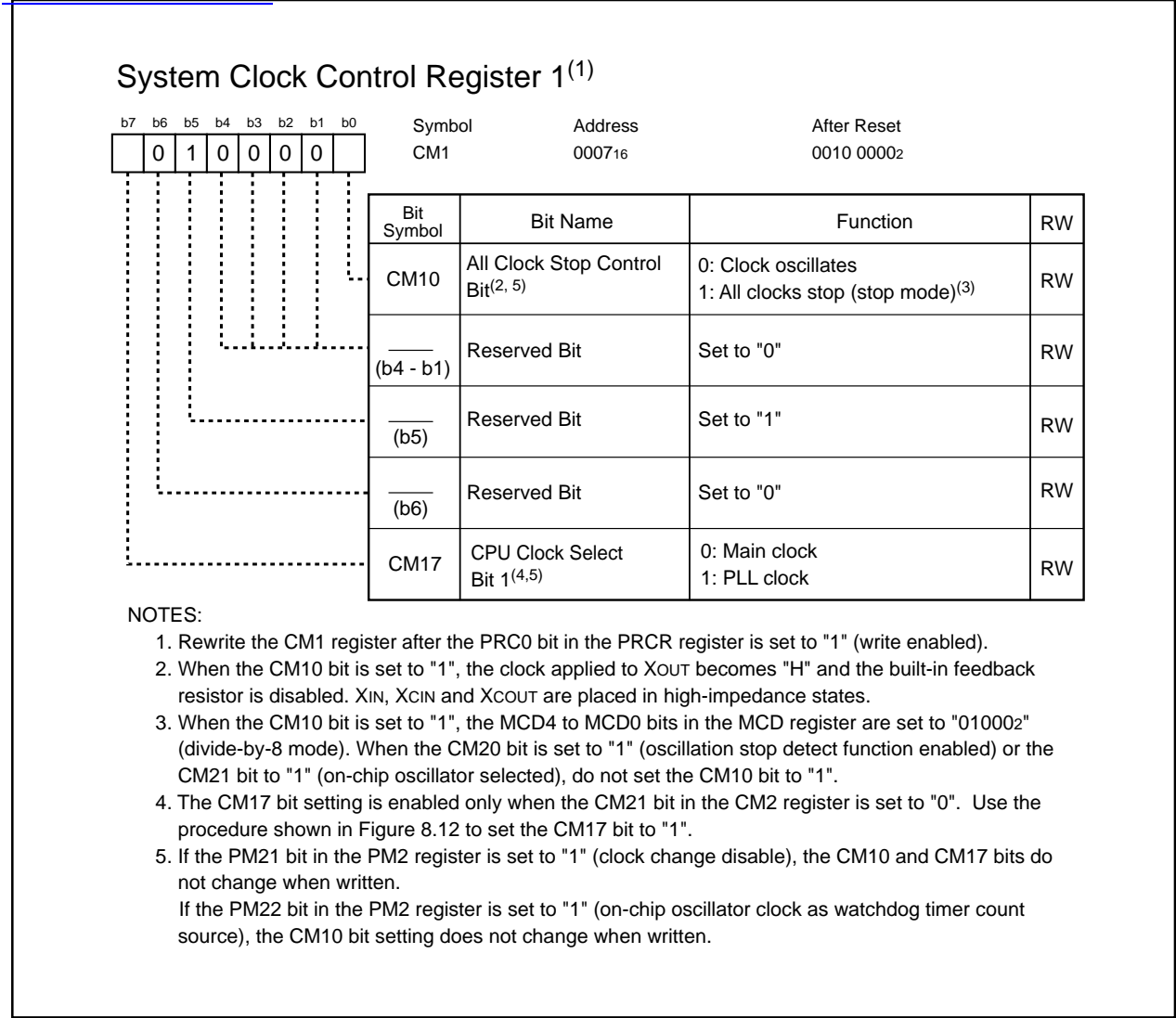
Figure 8.3 CM1 Register
