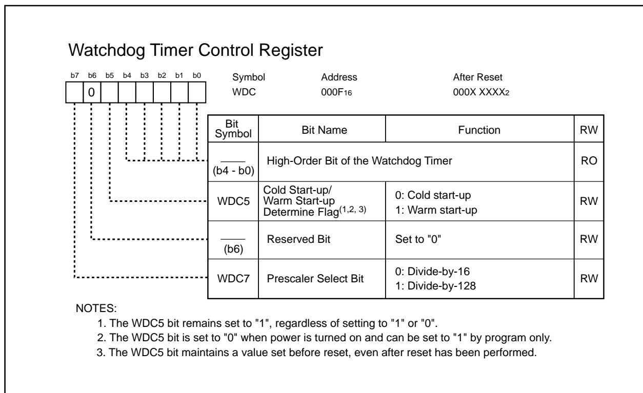
Figure 6.1 WDC Register
