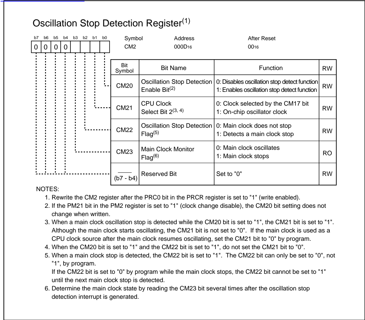
Figure 8.5 CM2 Register
