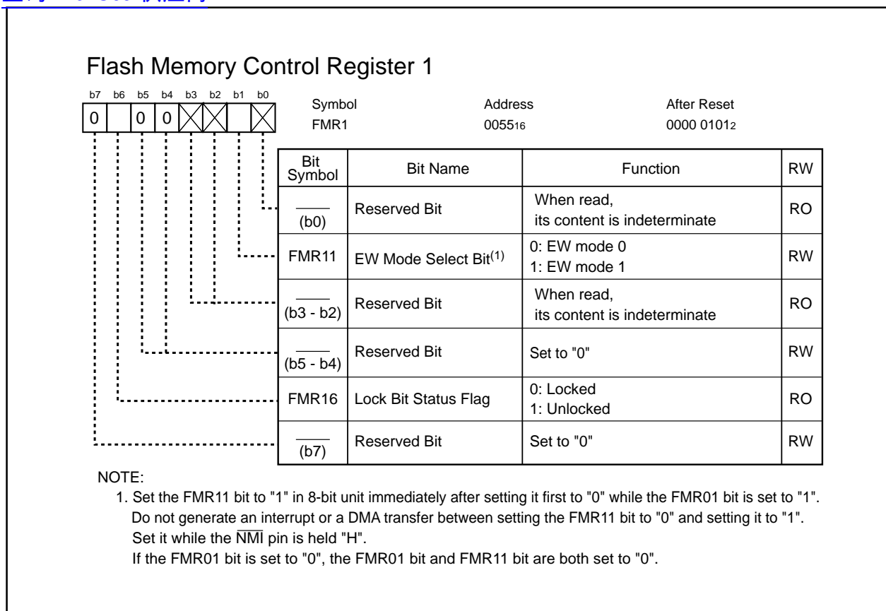
Figure 24.5 FMR1 Register
