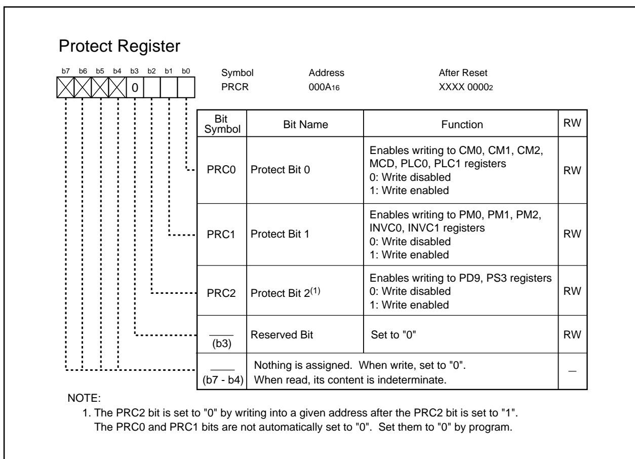
Figure 9.1 PRCR Register
