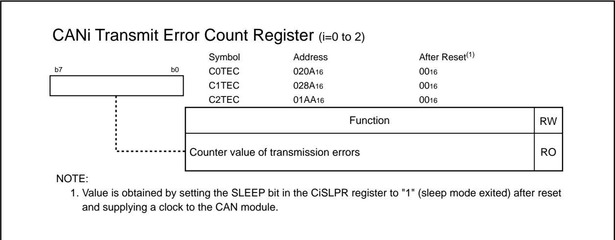
Figure 22.11 C0TEC, C1TEC and C2TEC Registers
