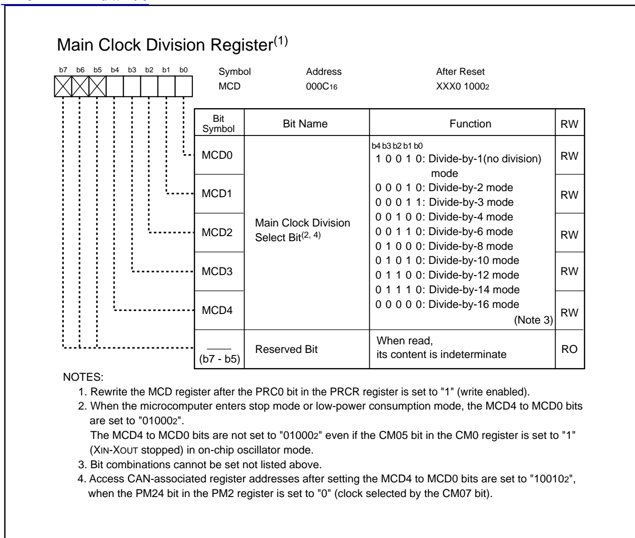
Figure 8.4 MCD Register
