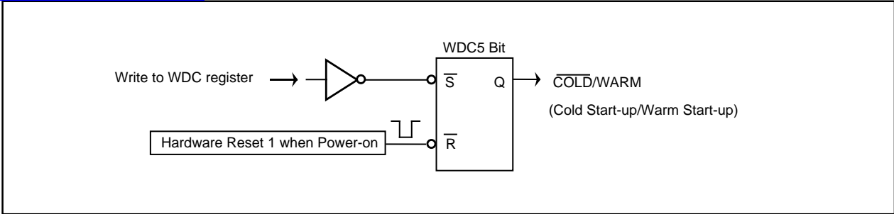
Figure 6.2 Cold Start-up/Warm Start-up Determine Function Block Diagram
