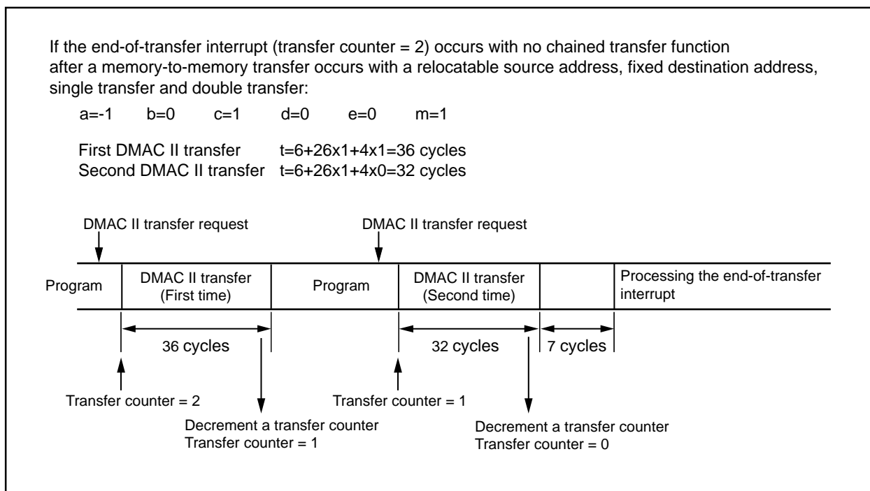
Figure 13.5 Transfer Cycle
