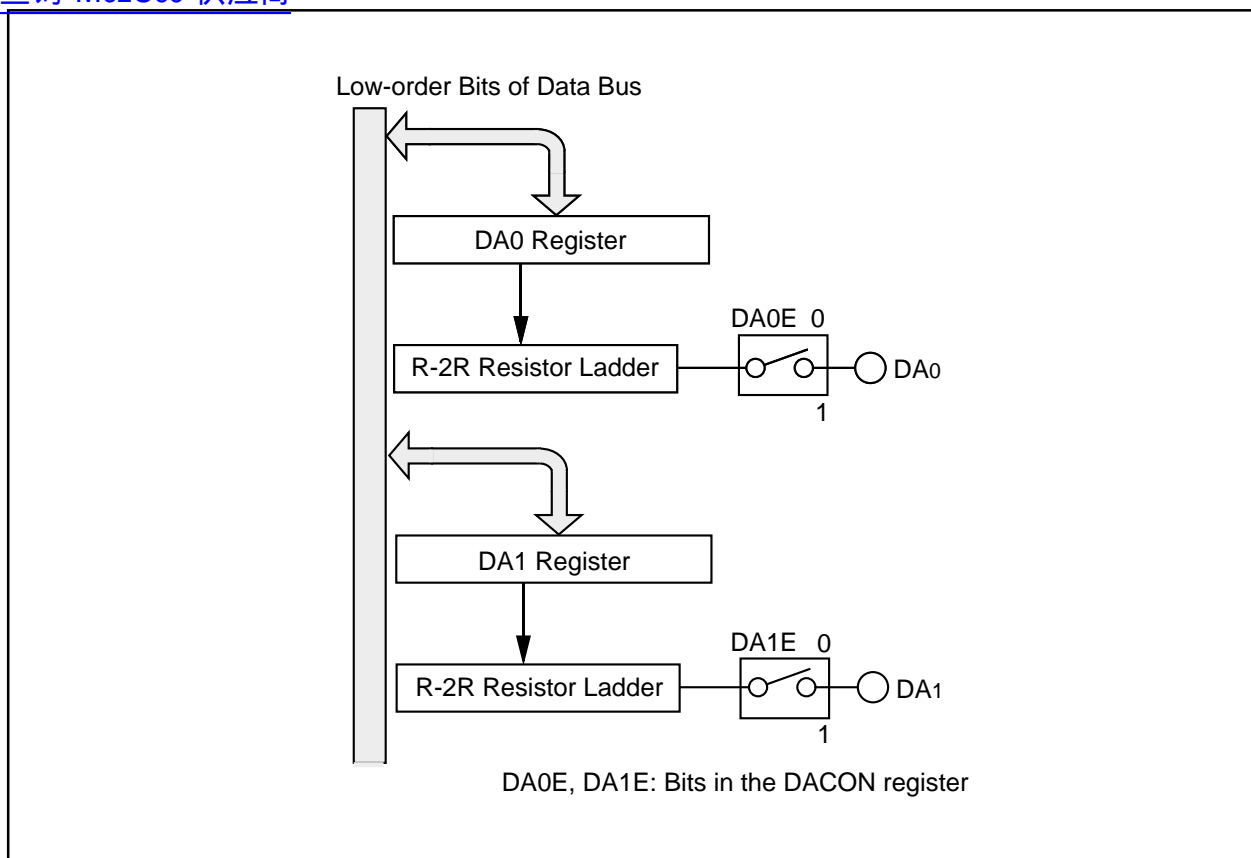
Figure 18.1 D/A Converter
