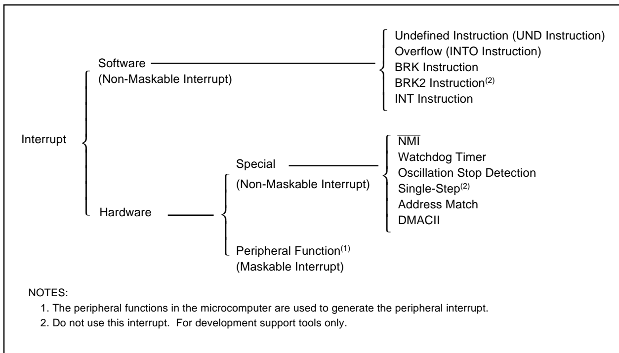
Figure 10.1 Interrupts
