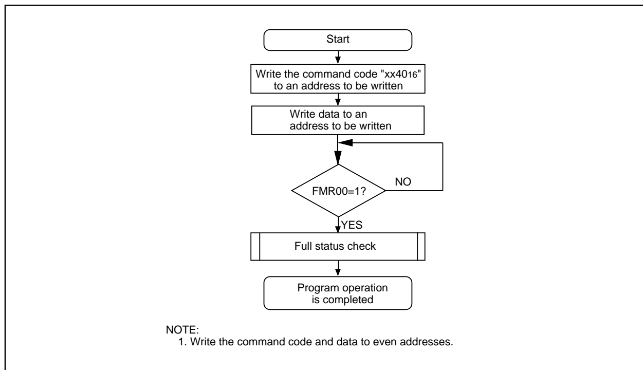
Figure 24.9 Program Command
