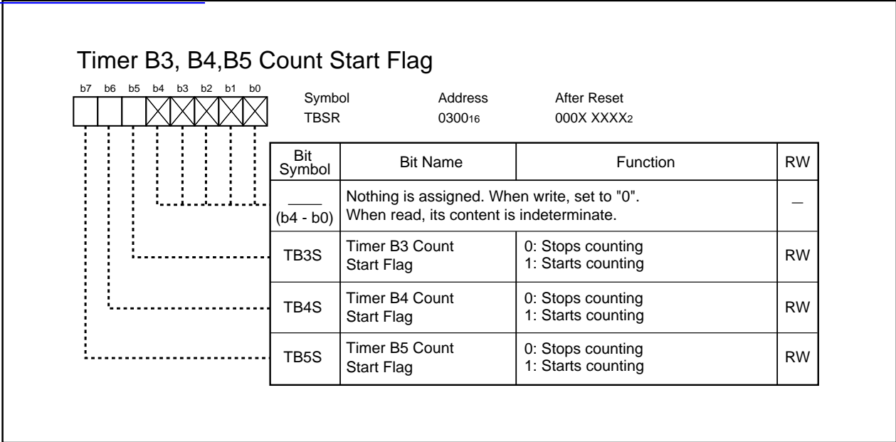
Figure 14.19 TBSR Register
