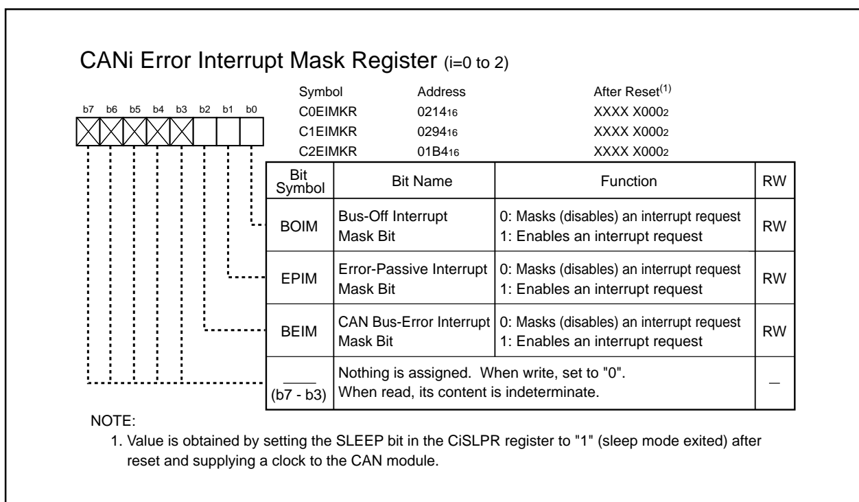
Figure 22.15 C0EIMKR, C1EIMKR and C2EIMKR Registers
