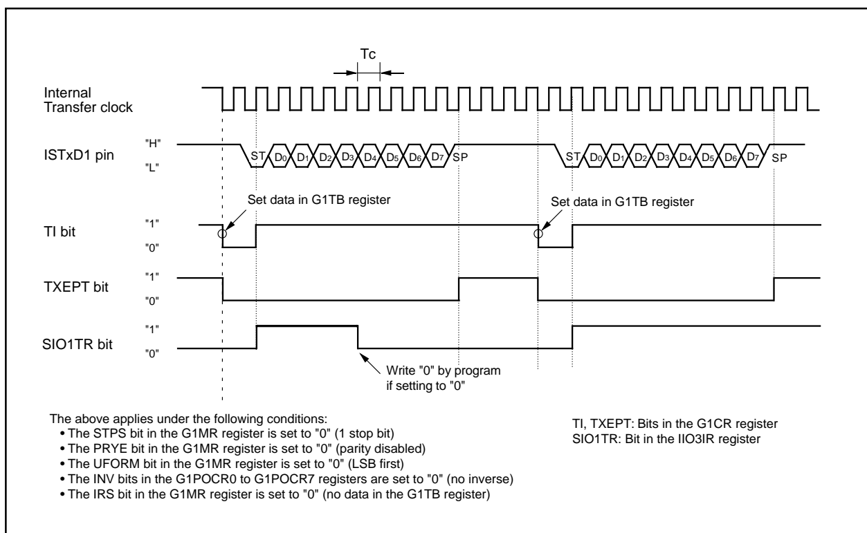
Figure 21.30 Transmit Operation
