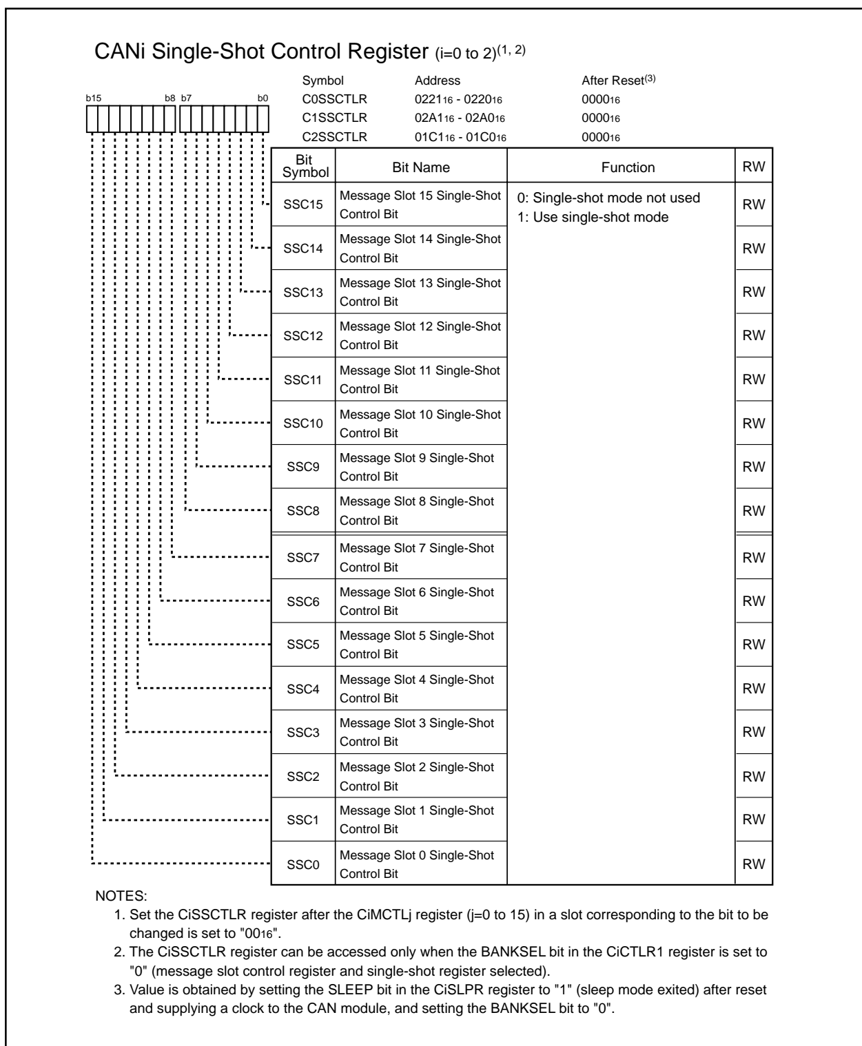
Figure 22.20 C0SSCTL R , C1SSCTL R and C2SSCTL R Registers
