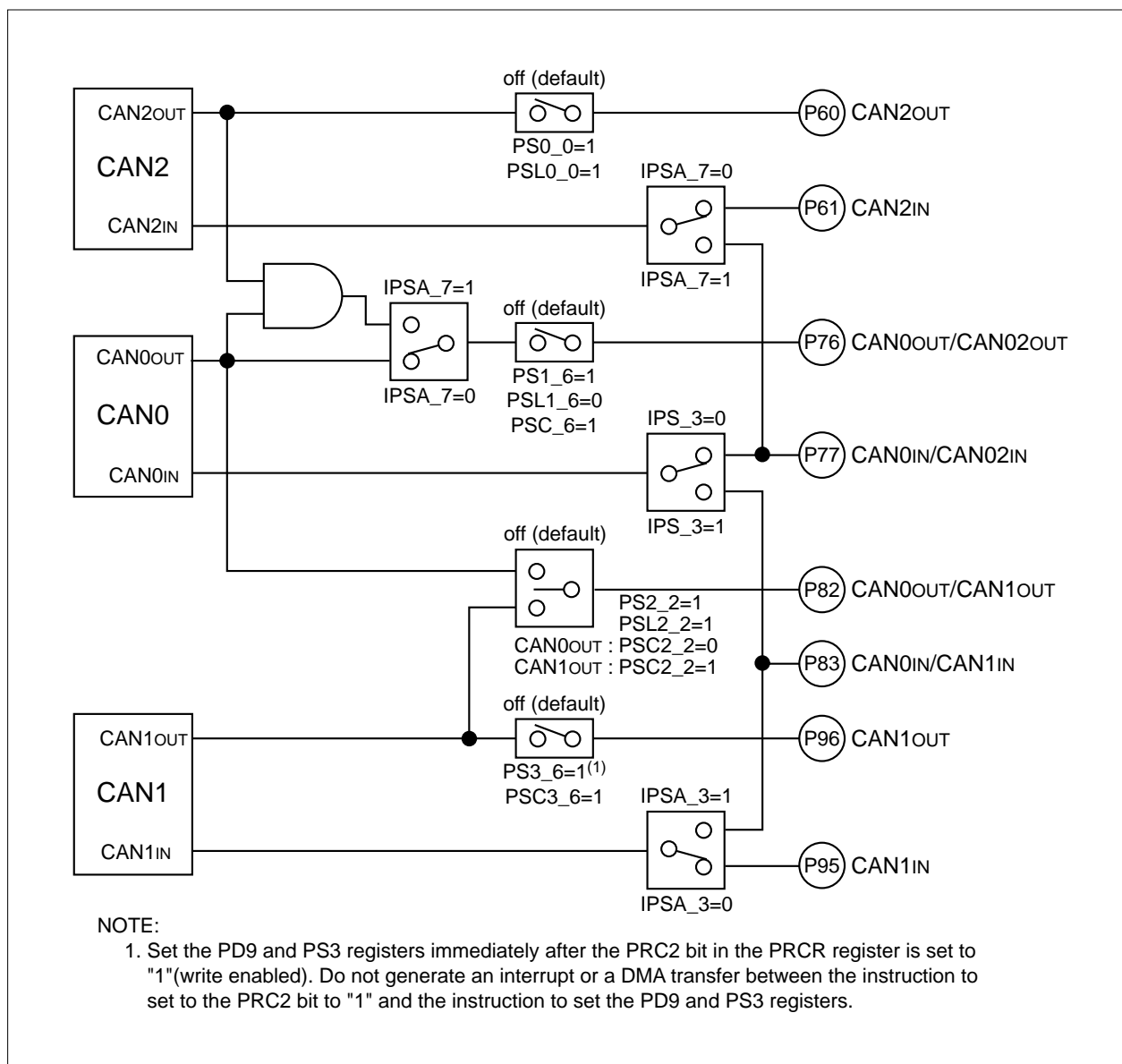
Figure 22.42 CAN0/CAN2 Combination Mode Block Diagram
