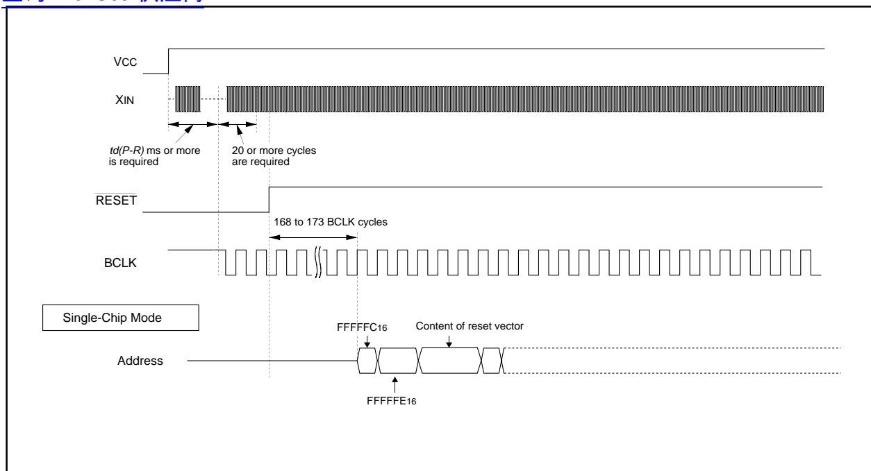
Figure 5.2 Reset Sequence
