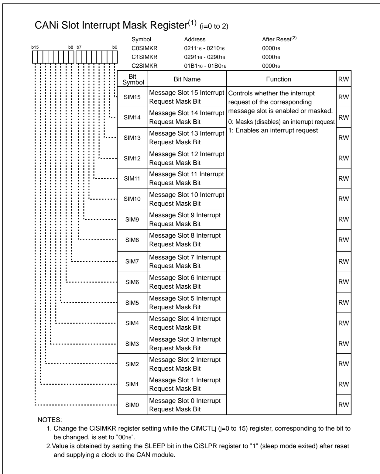
Figure 22.14 C0SIMKR, C1SIMKR and C2SIMKR Registers
