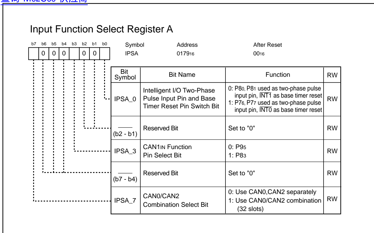
Figure 23.18 IPSA Register
