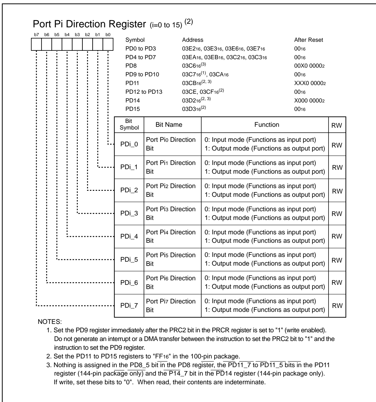
Figure 23.5 PD0 to PD15 Registers
