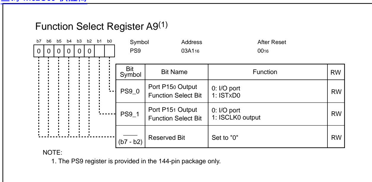
Figure 23.10 PS9 Register
