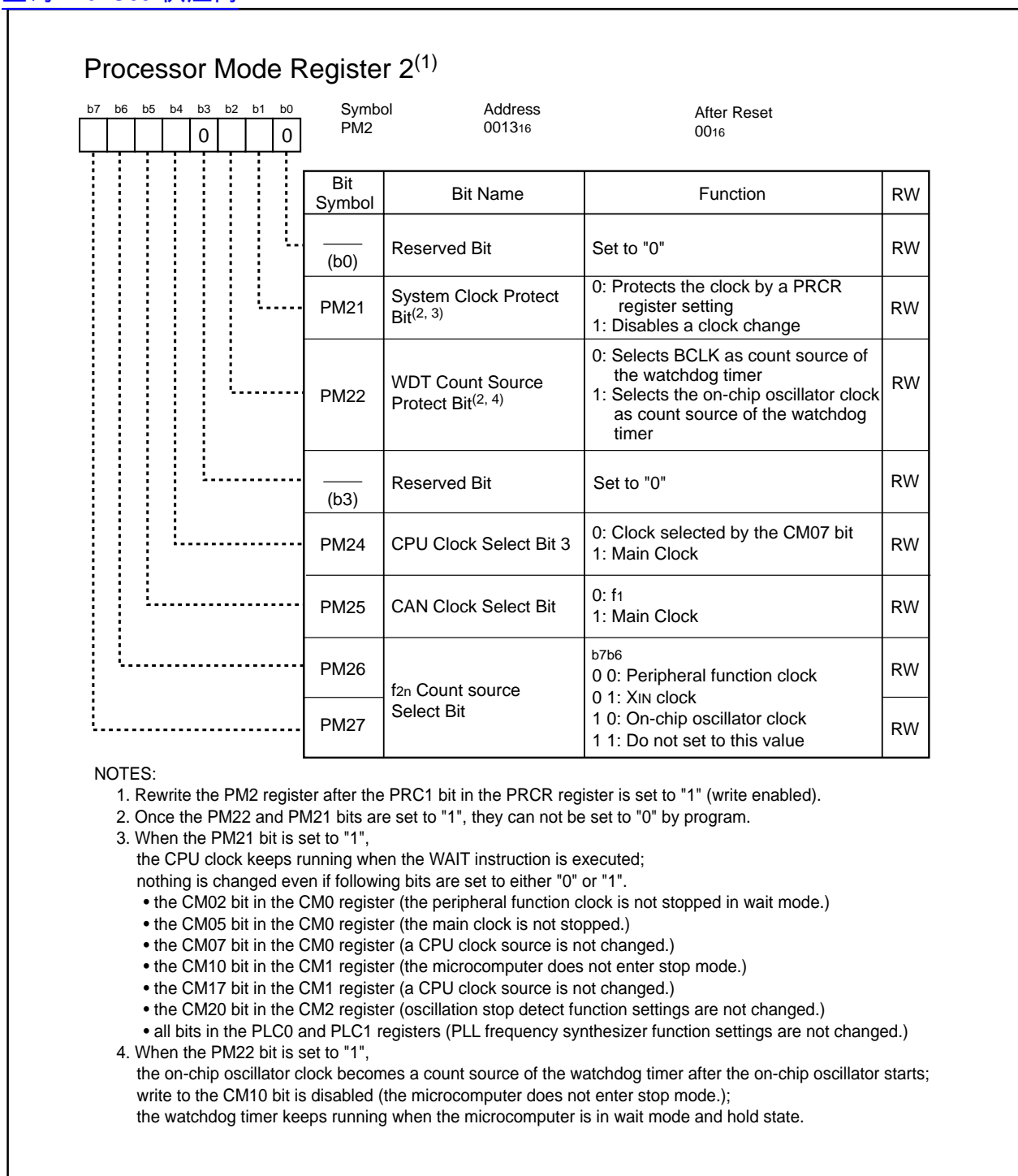
Figure 8.8 PM2 Register
