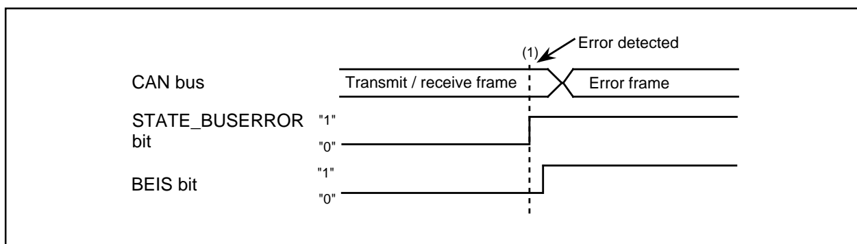
Figure 22.40 Operation Timing when CAN Bus Error Occurs
