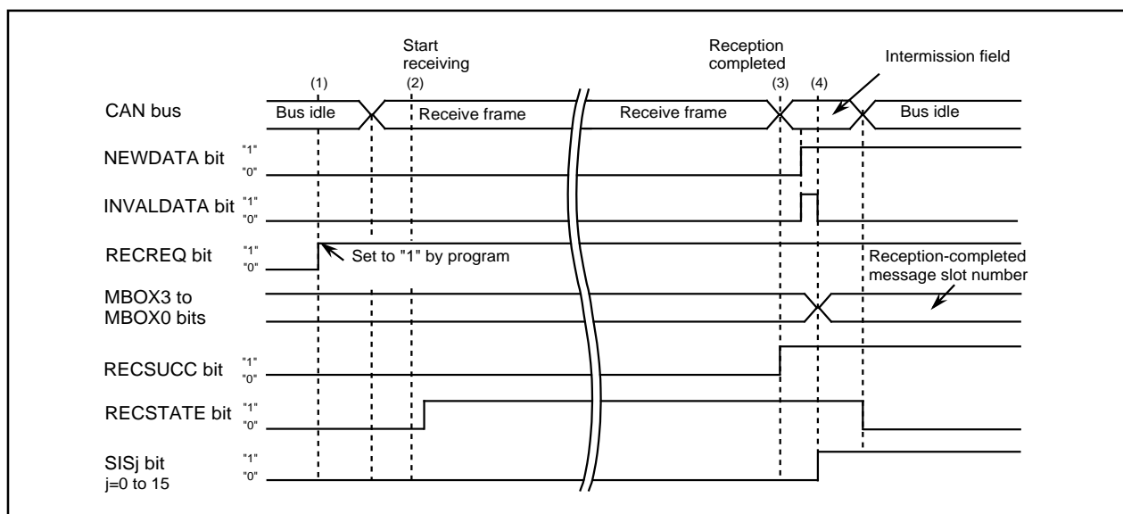
Figure 22.39 Example of CAN Data Frame Receive Operation
