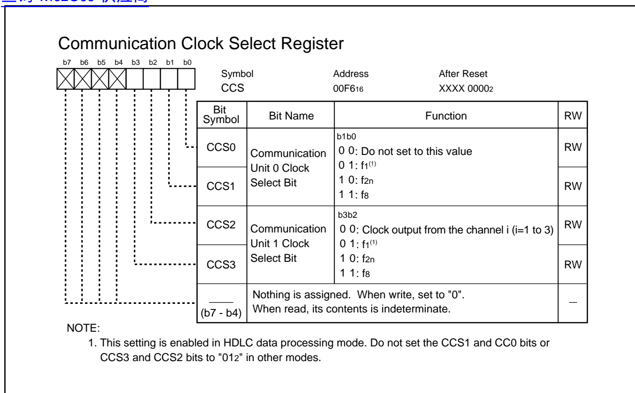
Figure 21.28 CCS Register
