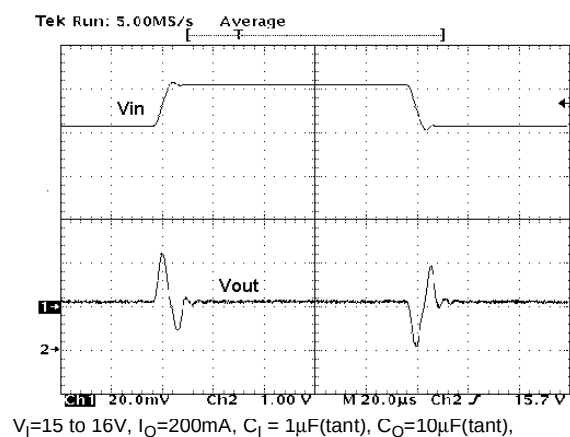
Figure 21 : Line Transient
