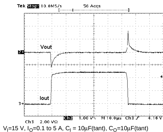
Figure 23 : Load Transient
