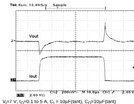
Figure 23 : Load Transient
