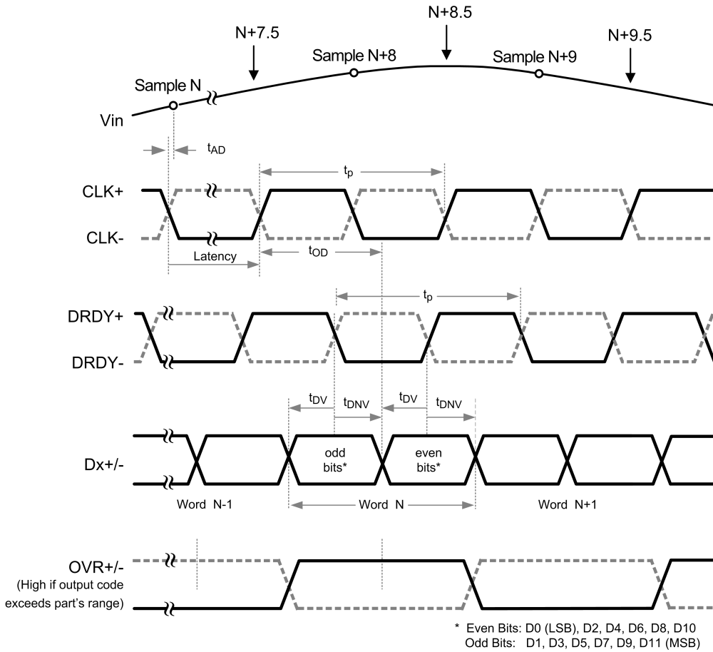
Output Timing
