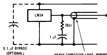
FIGURE 4. LM34 with R-C Damper
