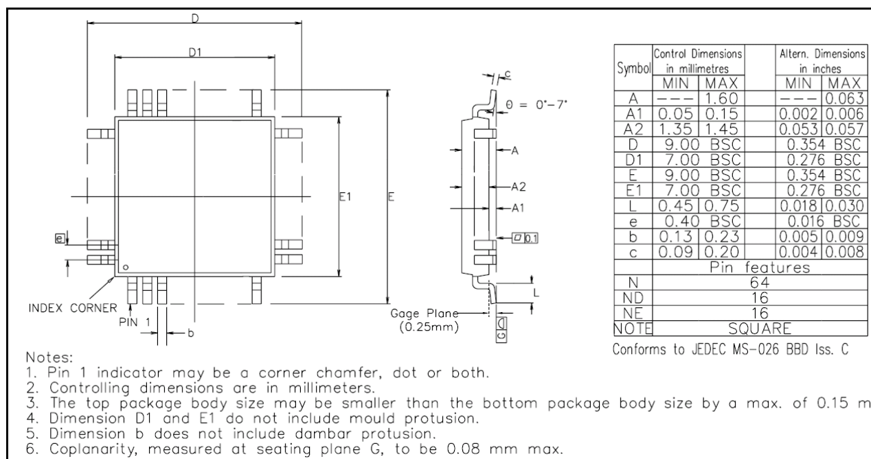
Figure 16 - Package dimensions
