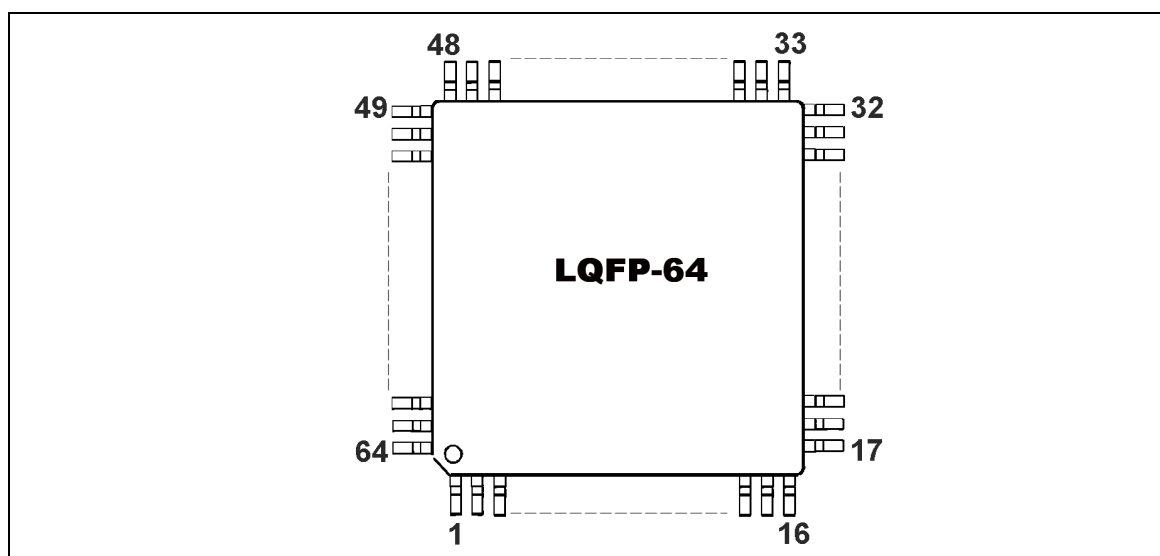
Figure 2 - CE6313 Pin Allocation
